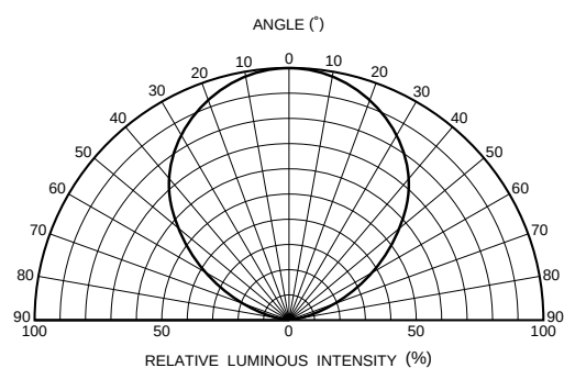
Fig.1 Directional pattern
