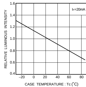
Fig.9 Luminous intensity vs. case temperature
