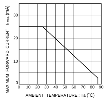
Fig.13 Maximum forward current vs. ambient temperature (Derating)
