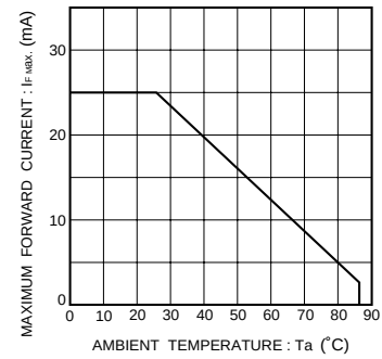
Fig.19 Maximum forward current vs. ambient temperature (Derating)
