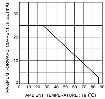
Fig.25 Maximum forward current vs. ambient temperature (Derating)
