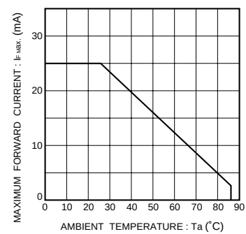
Fig.31 Maximum forward current vs. ambient temperature (Derating)
