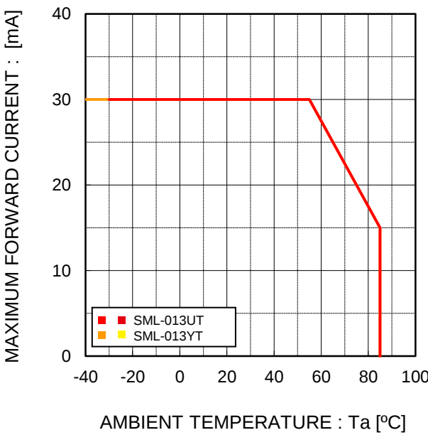
Fig.4 Derating
