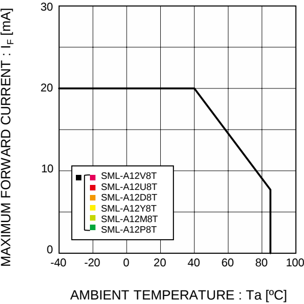
Fig.4 Derating
