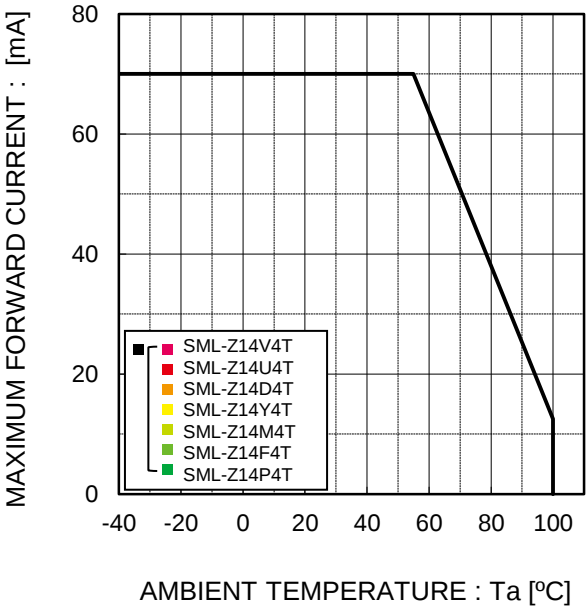
Fig.4 Derating
