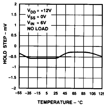
Hold Step vs. Temperature
