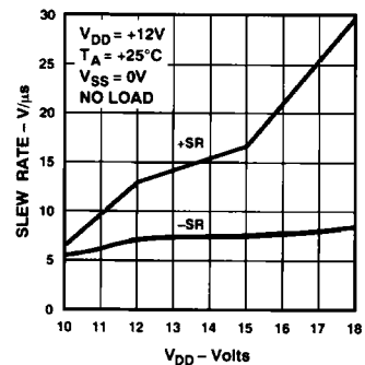
Slew Rate vs. V_{DD}
