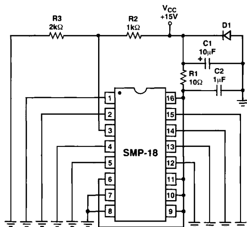
Burn-in Circuit
