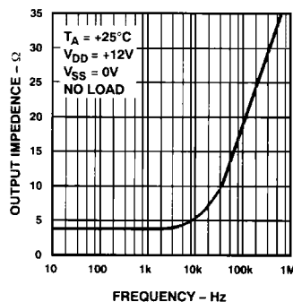
Output Impedance vs. Frequency
