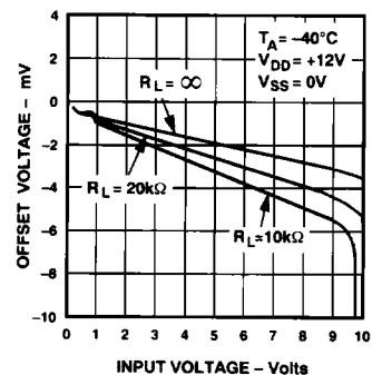
Offset Voltage vs. Input Voltage
