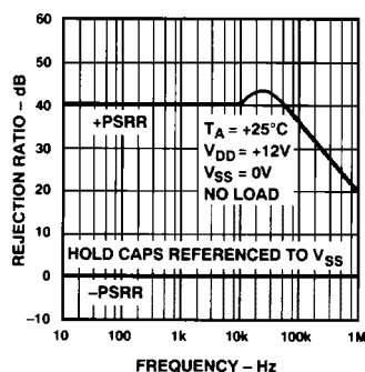
Hold Mode Power Supply Rejection
