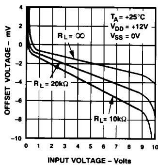
Offset Voltage vs. Input Voltage
