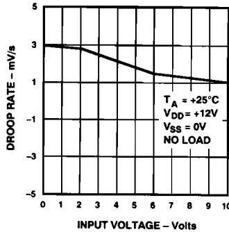
Droop Rate vs. Input Voltage
