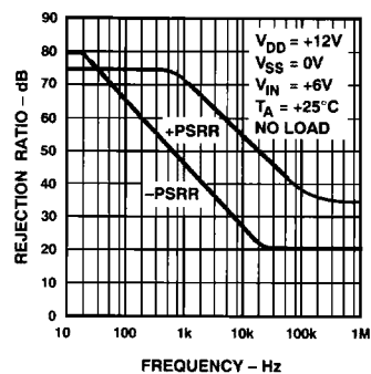
Sample Mode Power Supply Rejection
