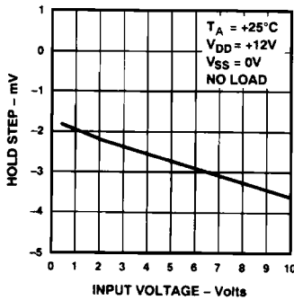
Hold Step vs. Input Voltage
