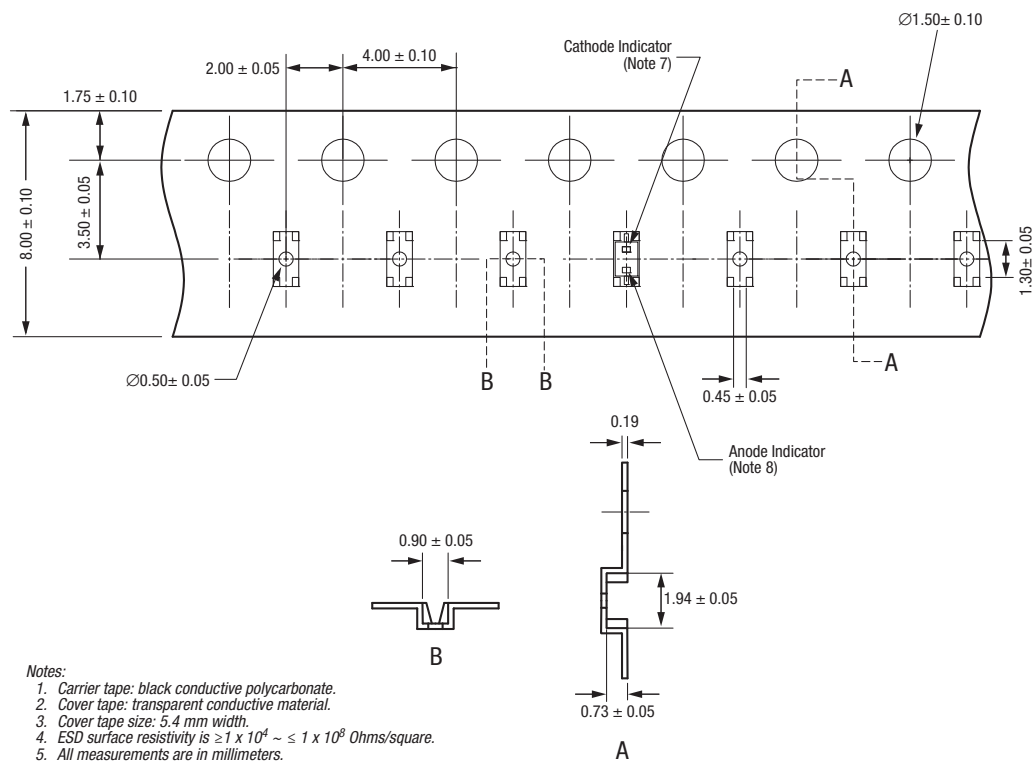
Figure 6. SC-79 Tape and Reel Dimensions
