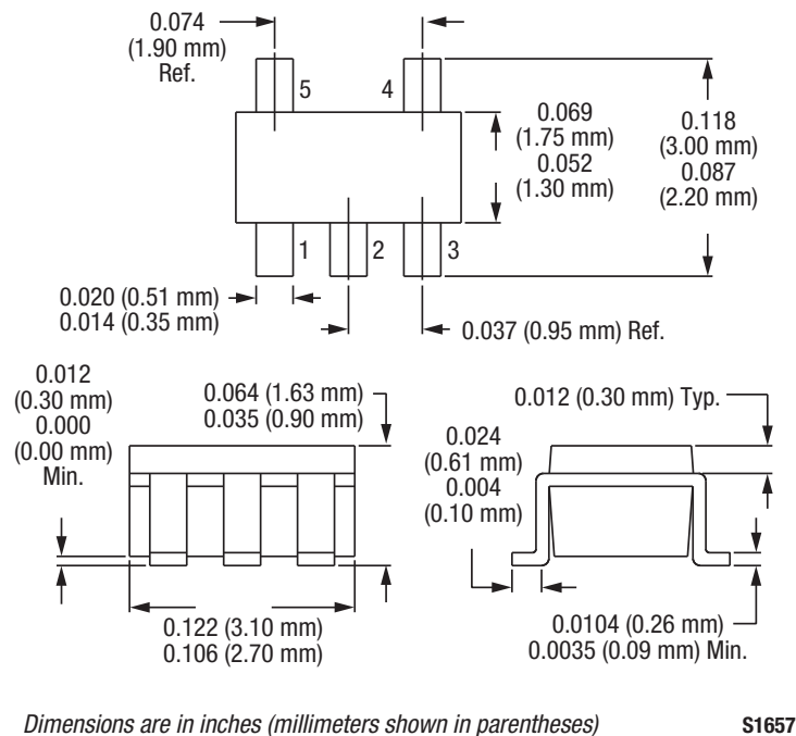
Figure 7. SOT-5 Package Dimension Drawing
