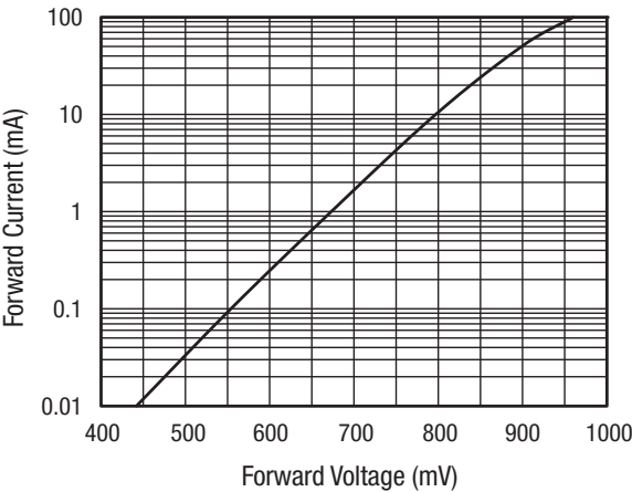
Figure 2. DC Characteristic
