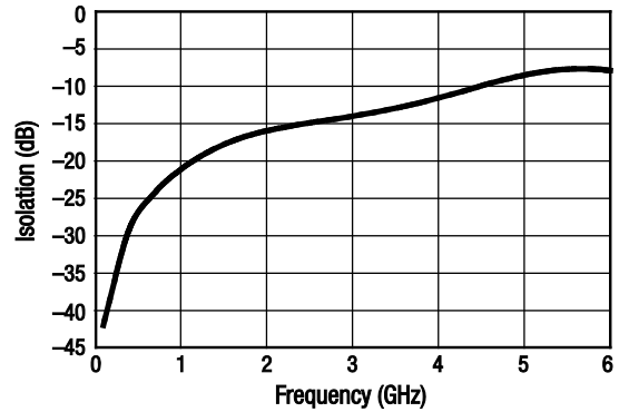
Figure 4. Isolation vs Frequency (I F = 0 mA)
