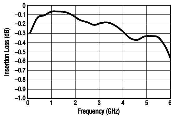
Figure 3. Insertion Loss vs Frequency (I F = 10 mA)
