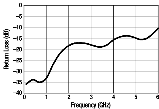
Figure 5. Return Loss vs Frequency (I F = 10 mA)
