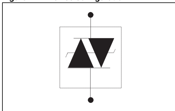
Figure 1. Device configuration
