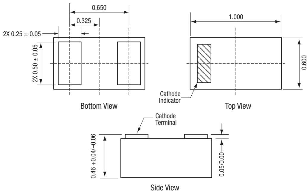
Figure 9. SOD-882 Package Dimensions
