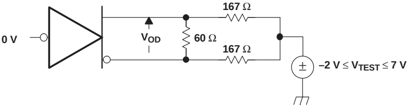
Figure 2. Driver V_{OD}
