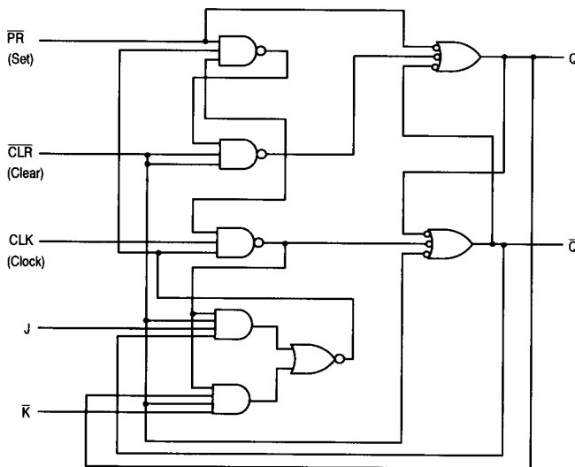
LOGIC DIAGRAM (one half shown)
