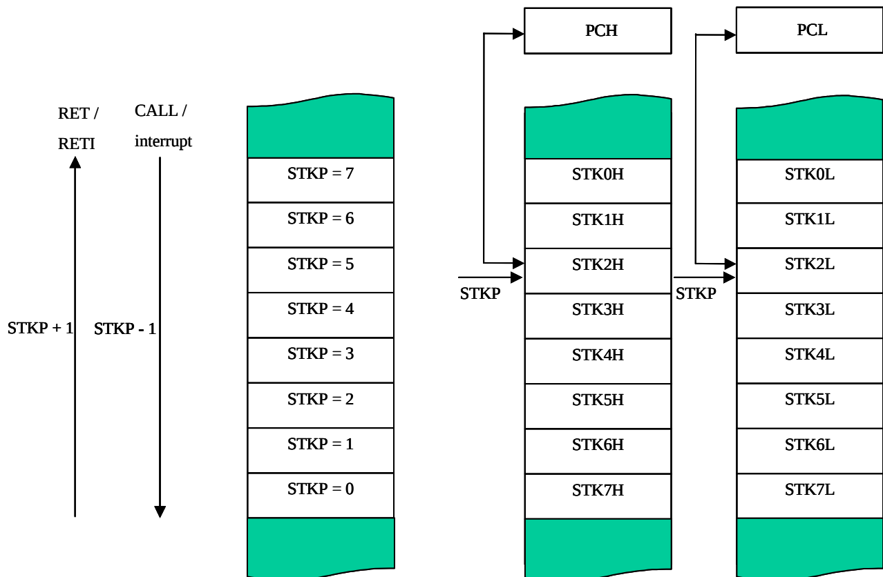
Figure 3-7 Stack-Save and Stack-Restore Operation
