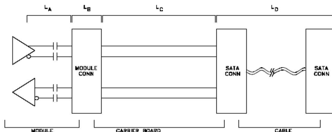
Figure 18: SATA Insertion Loss Budge
