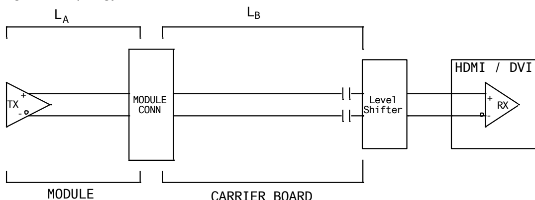
Figure 9: Topology for HDMI / DVI
