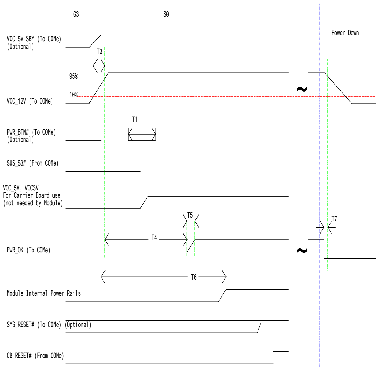
Figure 31: AT Style Power Up Boot
