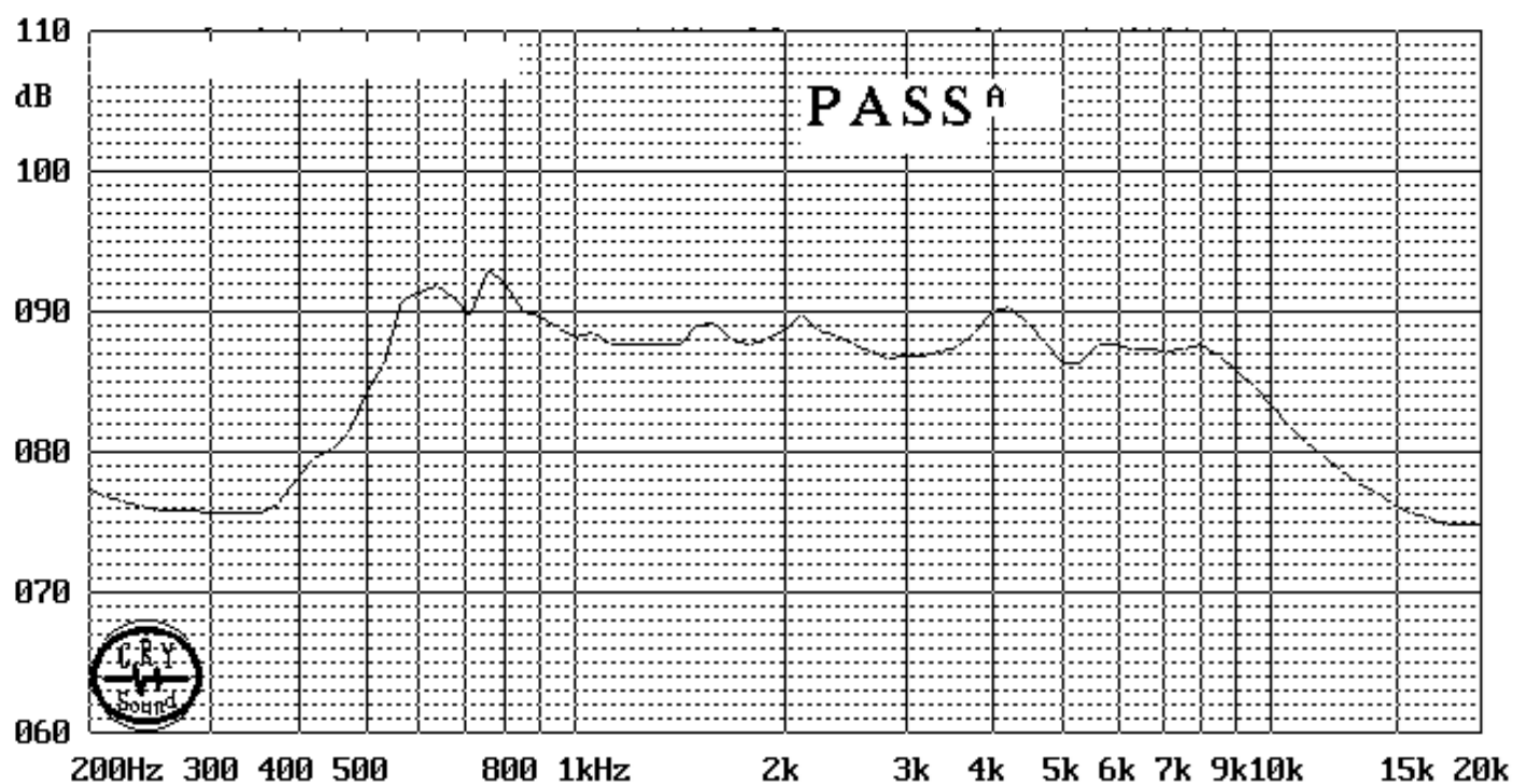
TYPICAL FREQUENCY RESPONSE CURVE (Figure 2)
