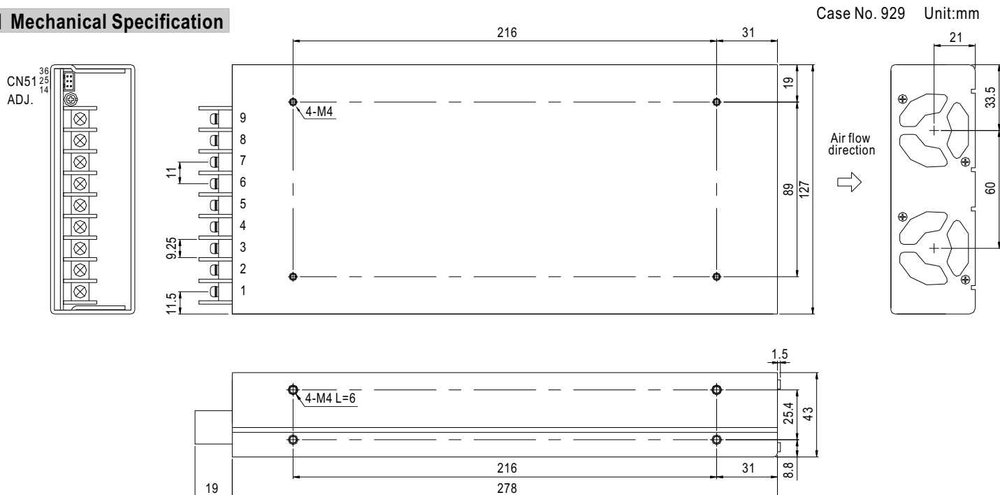
Terminal pin number assignment :
