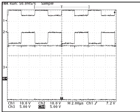
Figure 2, SP233A Charge pump waveforms- no load (1 = C1+, 2 = C2+, 3 = V+, 4 = V-).
