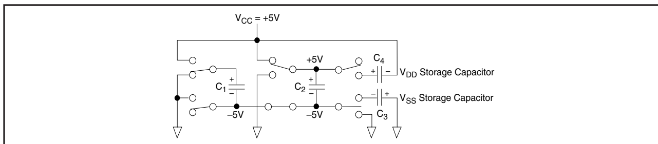
Figure 5. Charge Pump - Phase 1
