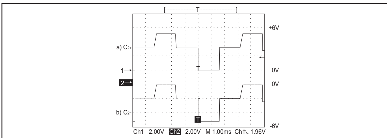
Figure 7. Charge Pump Waveforms
