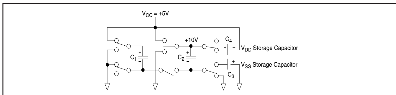
Figure 9. Charge Pump - Phase 4
