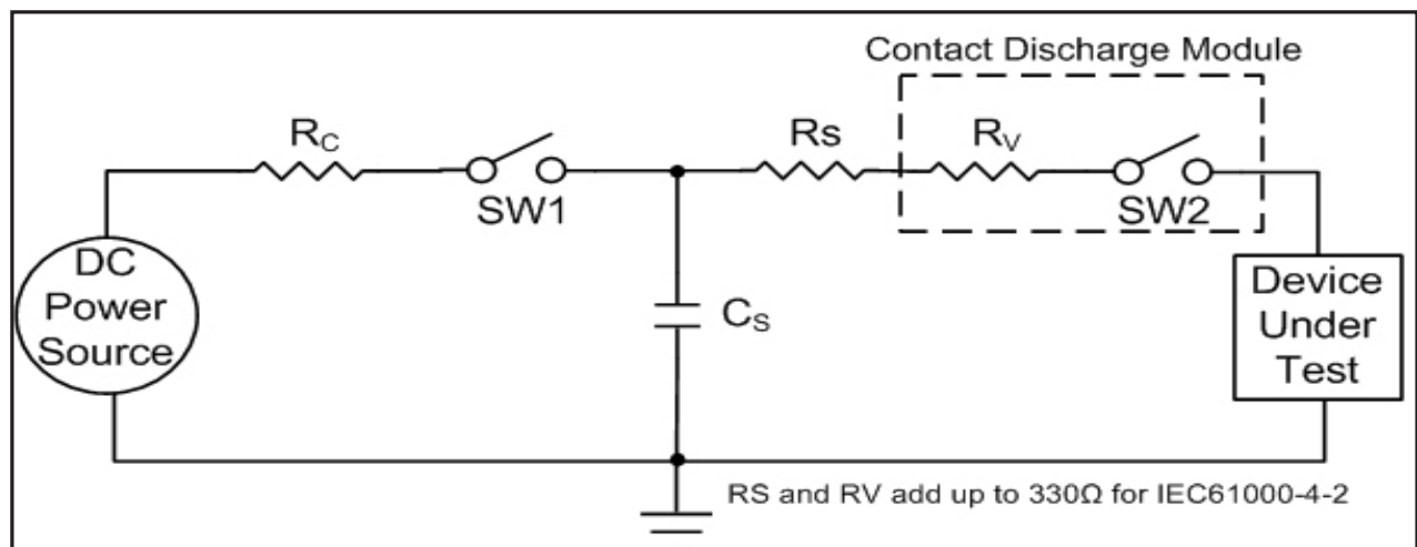
Figure 12. ESD Test Circuit for IEC61000-4-2
