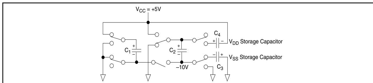
Figure 6. Charge Pump - Phase 2
