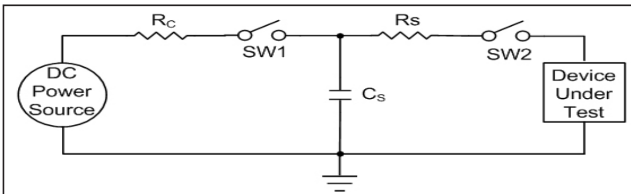
Figure 11. ESD Test Circuit for Human Body Model
