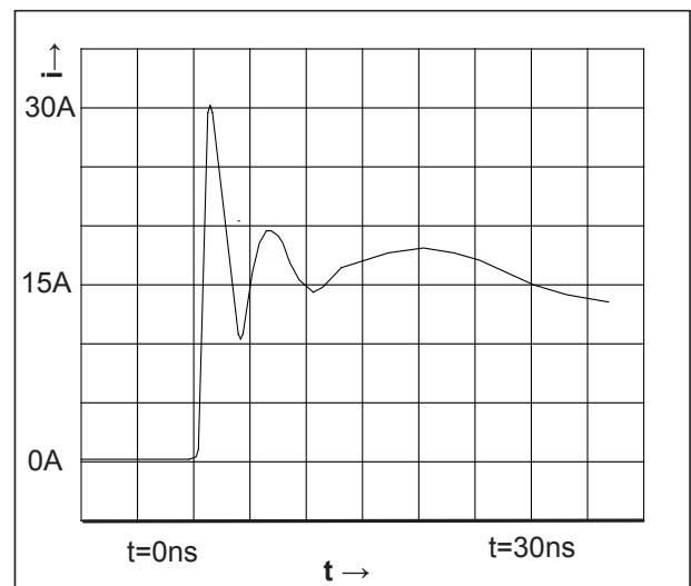
Figure 13. ESD Test Waveform for IEC61000-4-2
