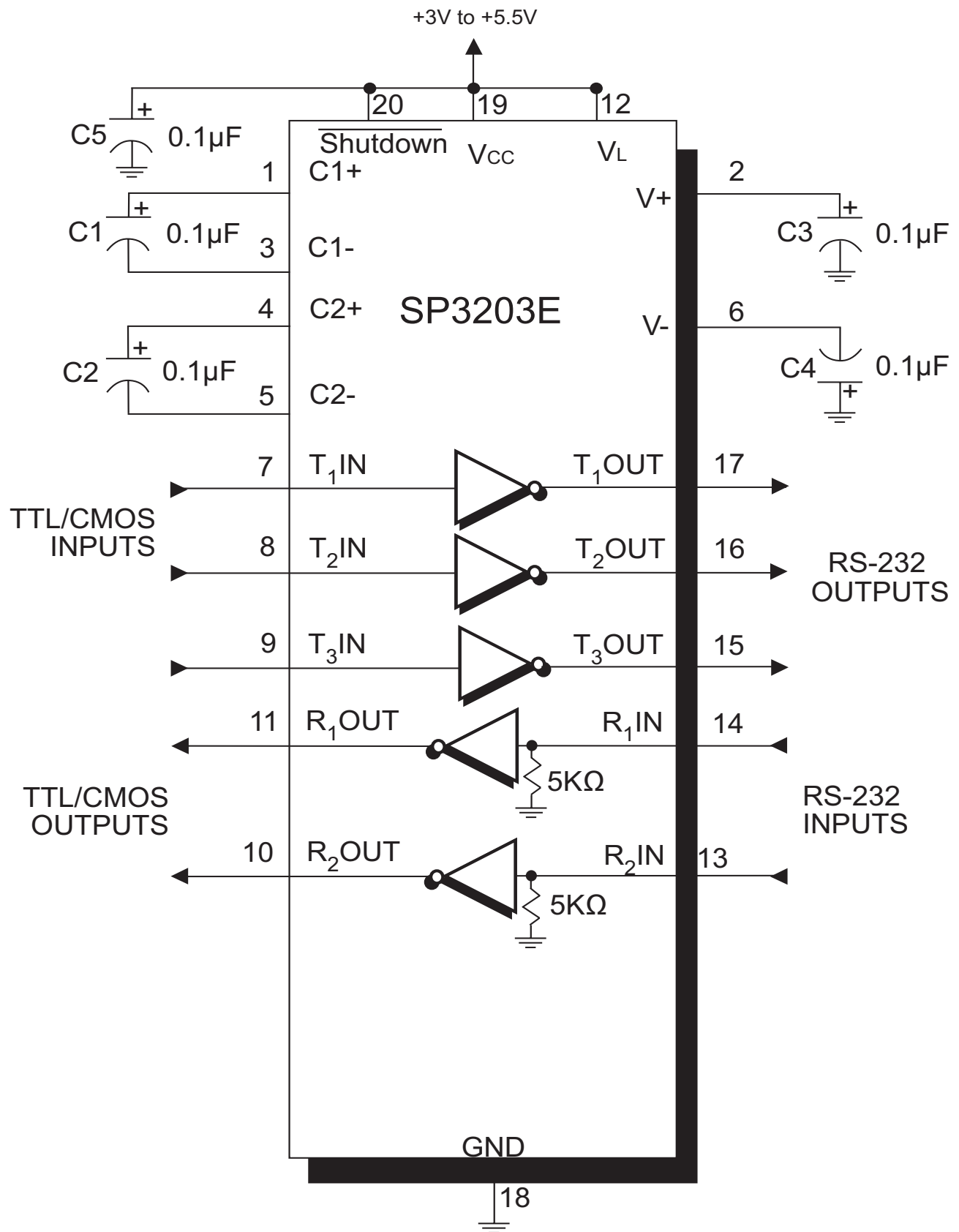
Figure 1. SP3203E Typical Operating Circuit
