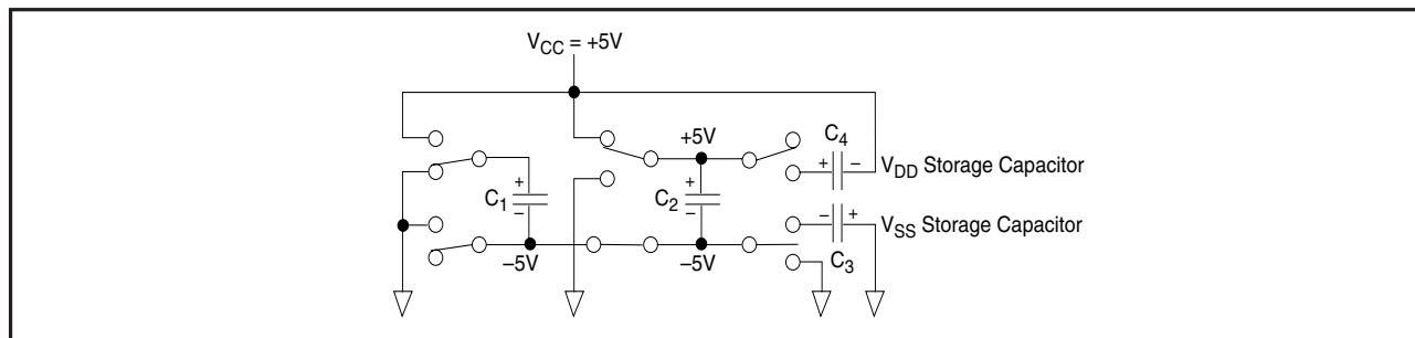
Figure 8. Charge Pump - Phase 3
