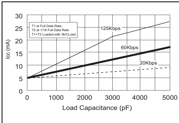
Figure 1. I_{cc} vs Load Capacitance for the SP3220EB.
