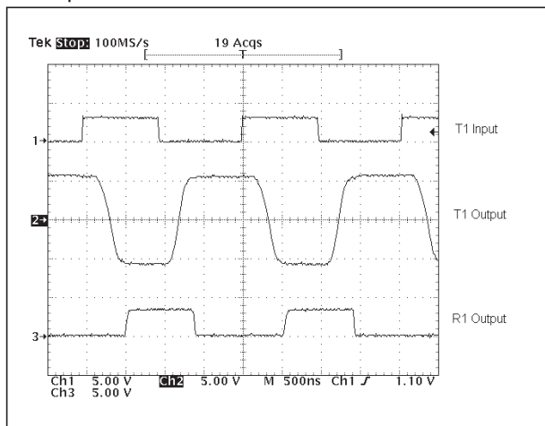
Figure 14. SP3220EU Loopback Test results at 1Mbps
