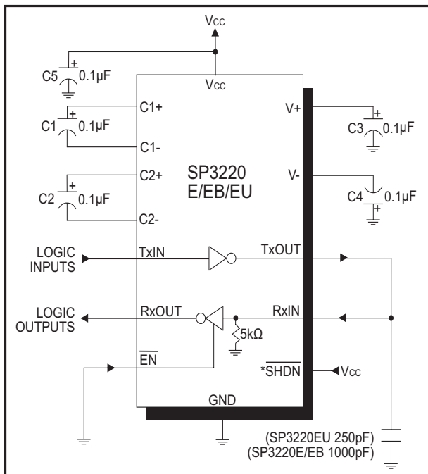
Figure 12. SP3220E/EB/EU Driver Loopback Test Circuit
