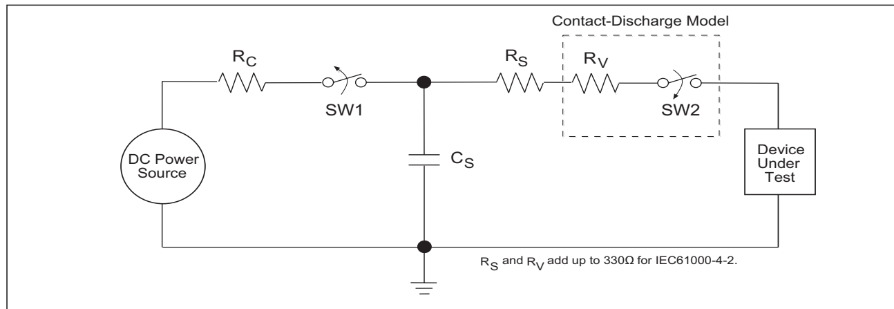
Figure 21. ESD Test Circuit for IEC61000-4-2
