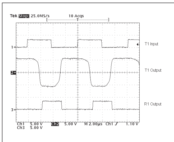
Figure 13. SP3220EB Loopback Test results at 250kbps
