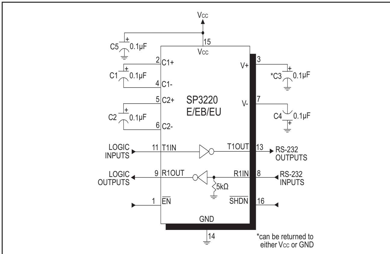
Figure 11. SP3220E/EB/EU Typical Operating Circuit
