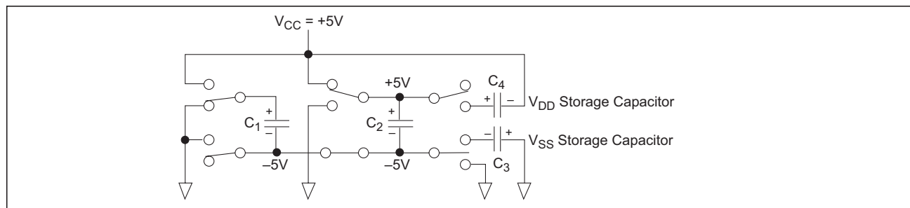
Figure 18. Charge Pump — Phase 3
