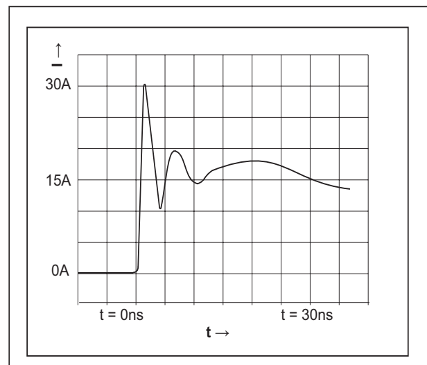
Figure 22. ESD Test Waveform for IEC61000-4-2
