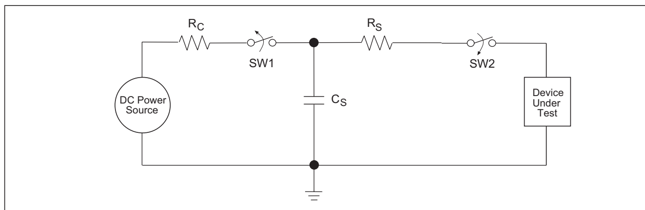
Figure 20. ESD Test Circuit for Human Body Model
