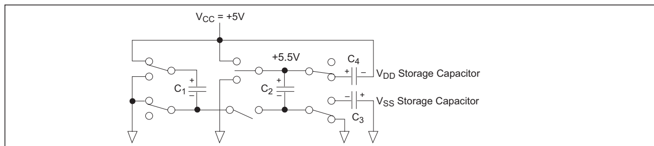
Figure 19. Charge Pump — Phase 4
