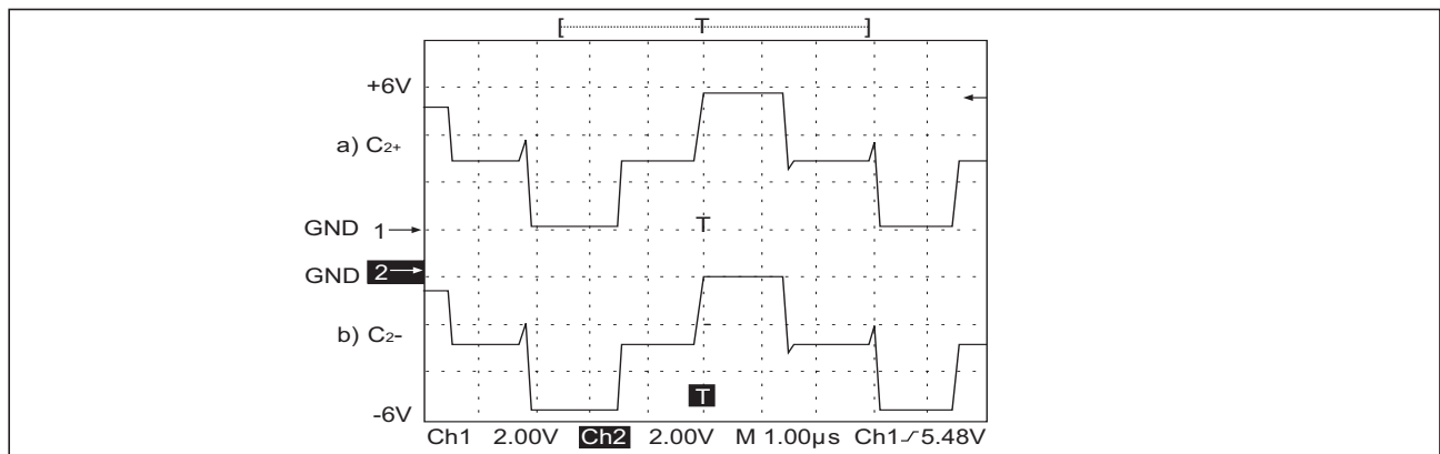
Figure 17. Charge Pump Waveforms
