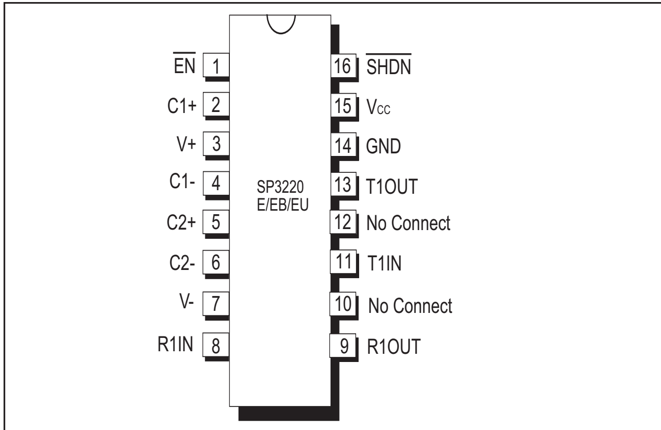
Figure 10. Pinout Configurations for the SP3220E/EB/EU
