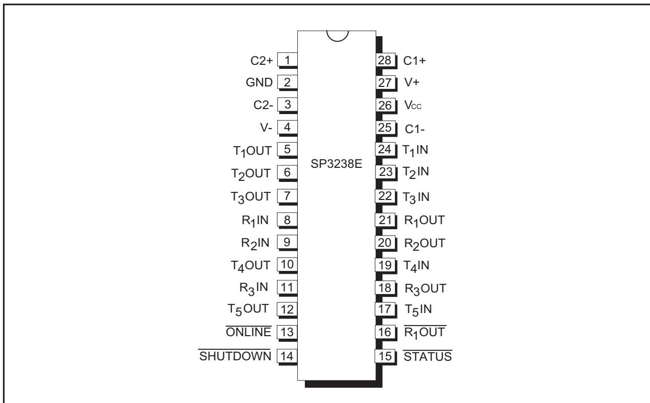
Figure 4. SP3238E Pinout Configuration
