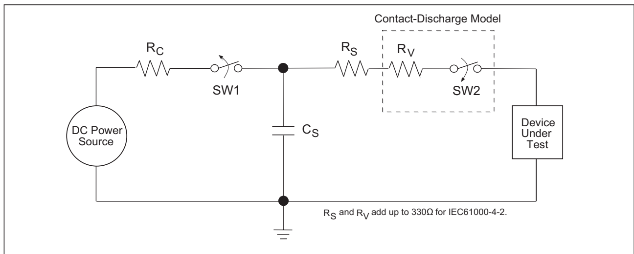
Figure 20. ESD Test Circuit for IEC61000-4-2
