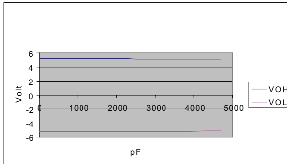
Figure 1. Transmitter Output Voltage VS. Load Capacitance
