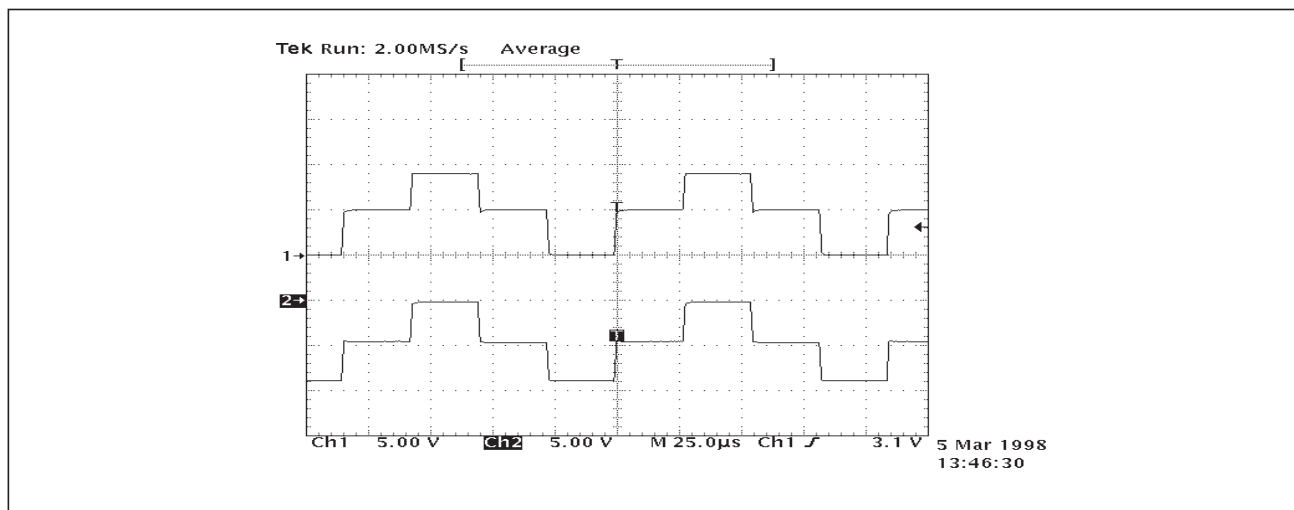
Figure 10. Charge Pump Waveform
