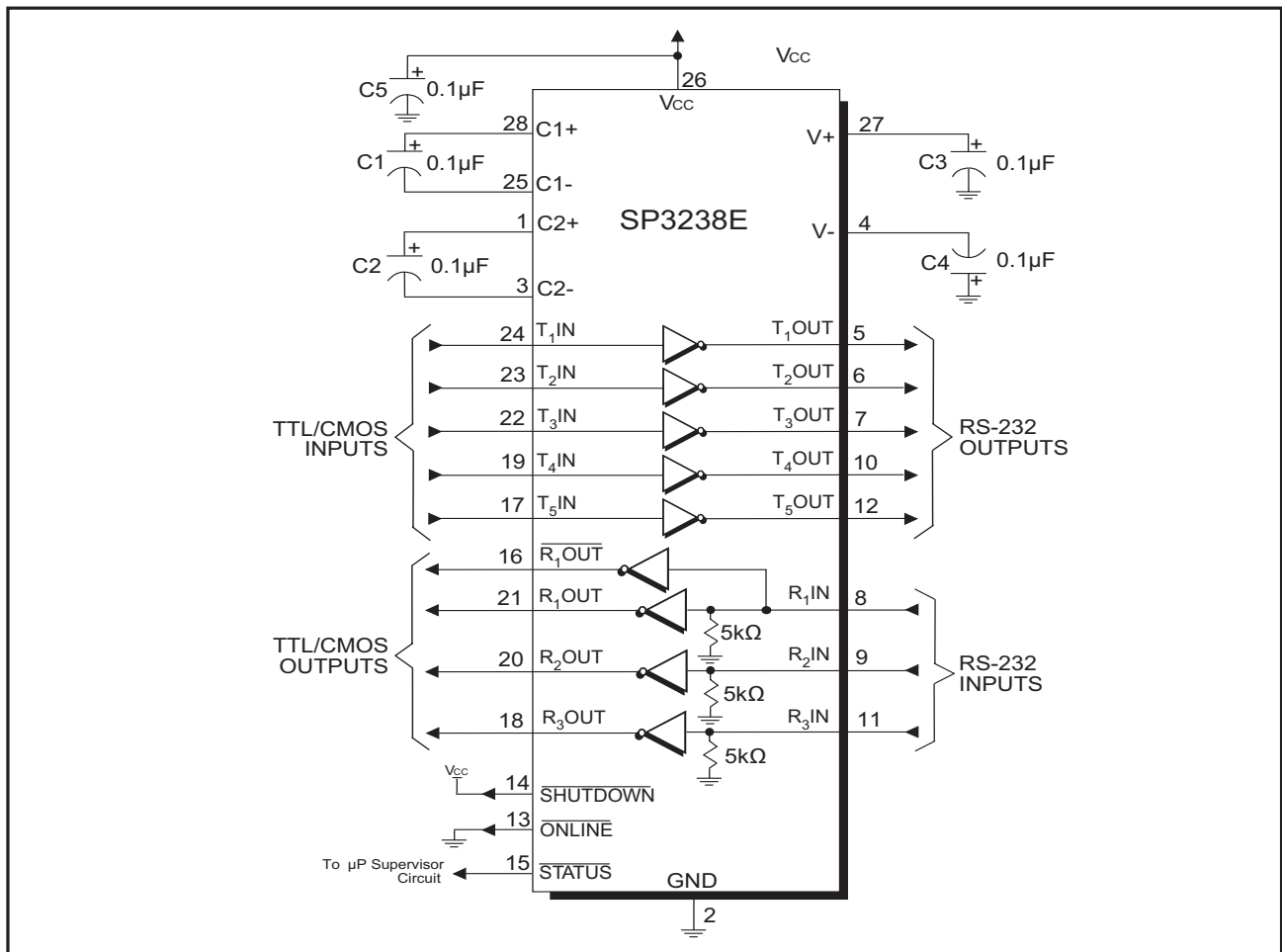
Figure 5. SP3238E Typical Operating Circuit
