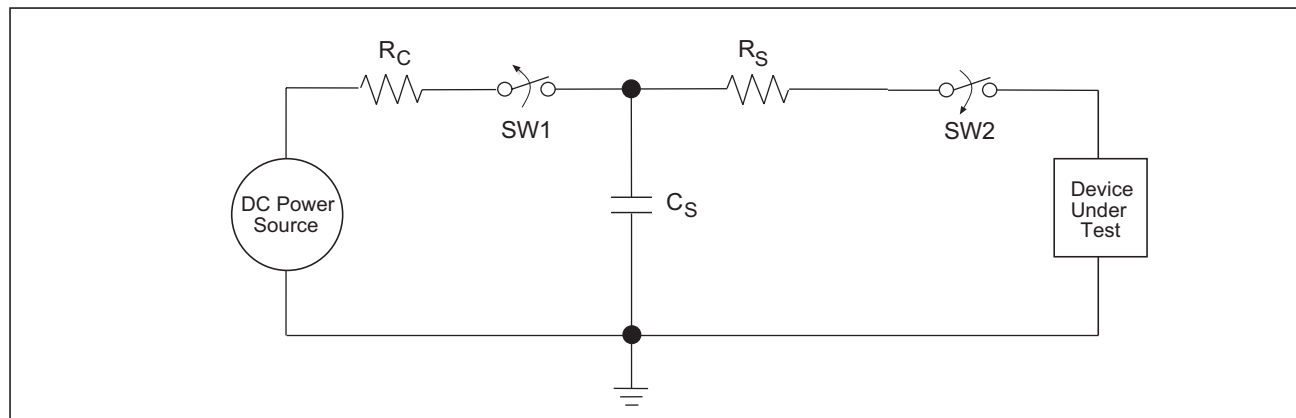
Figure 19. ESD Test Circuit for Human Body Model
