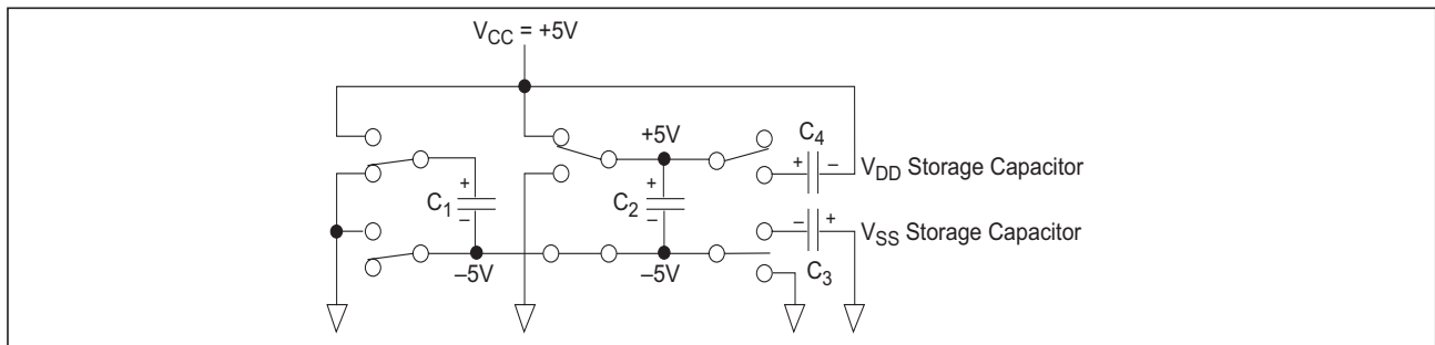
Figure 11. Charge Pump — Phase 1
