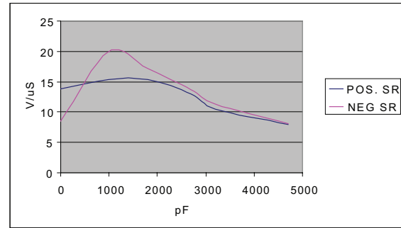
Figure 2. Slew Rate VS. Load Capacitance
