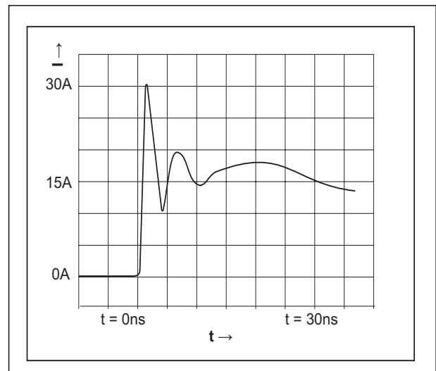
Figure 21. ESD Test Waveform for IEC61000-4-2
