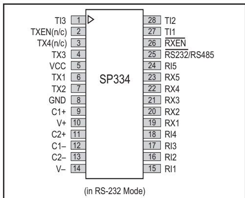
Figure 11. SP334 Pinout
