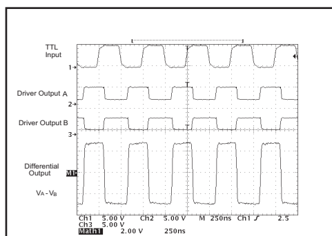
Figure 10. Typical RS-485 Driver Output
