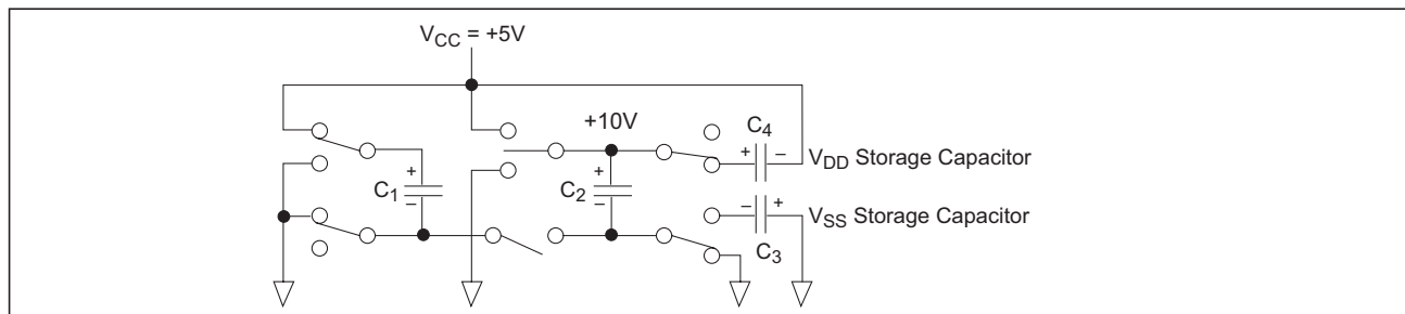
Figure 5. Charge Pump — Phase 4
