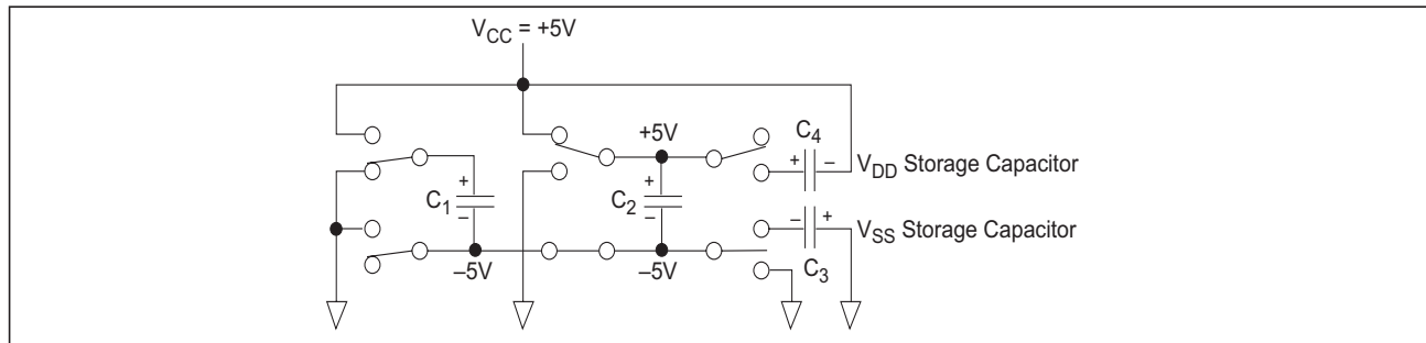
Figure 2. Charge Pump — Phase 1
