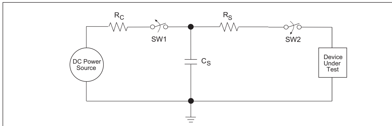
Figure 6. ESD Test Circuit for Human Body Model
