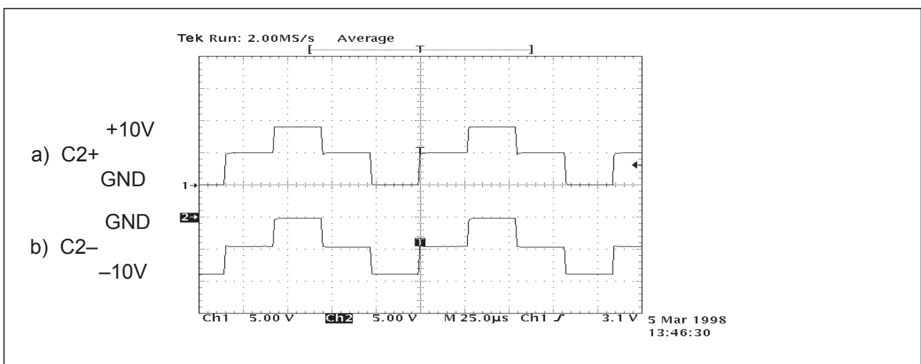
Figure 1. Charge Pump Waveform
