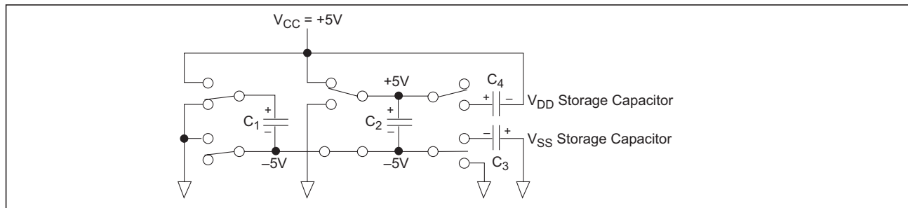
Figure 4. Charge Pump — Phase 3
