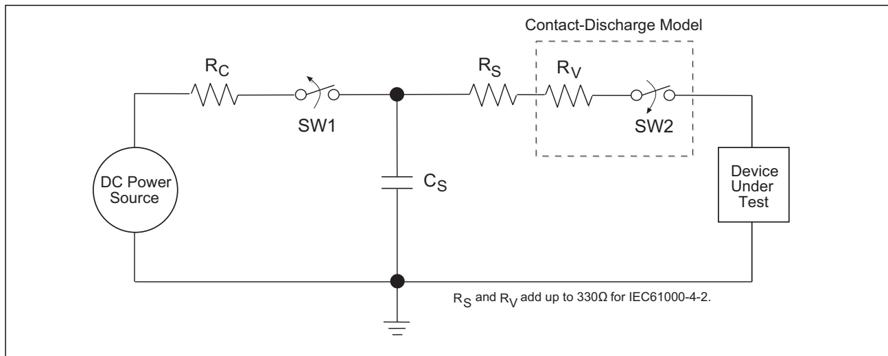
Figure 7. ESD Test Circuit for IEC61000-4-2
