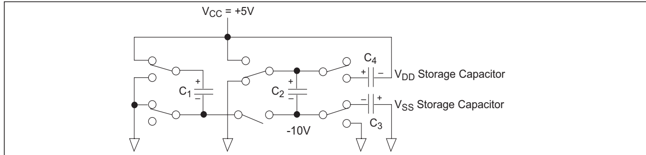
Figure 3. Charge Pump — Phase 2
