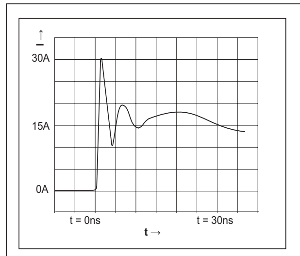
Figure 8. ESD Test Waveform for IEC61000-4-2
