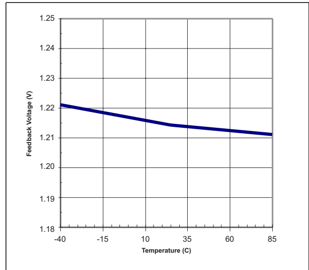
Figure 17. Feedback Voltage vs. Temperature
