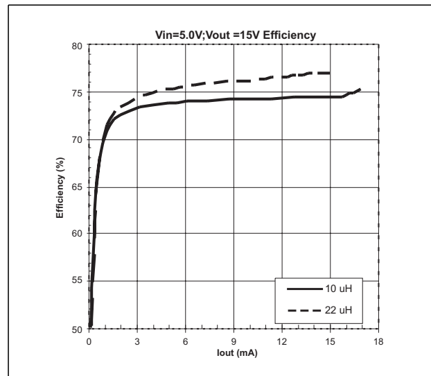
Figure 7. 15V Output Efficiency ( V_{IN}=5\text{V} )
