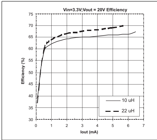
Figure 10. 20V Output Efficiency ( V_{IN}=3.3\text{V} )
