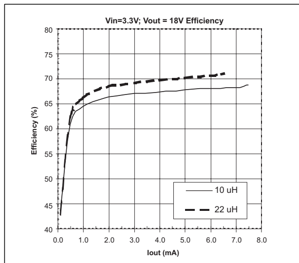
Figure 8. 18V Output Efficiency ( V_{IN}=3.3\text{V} )
