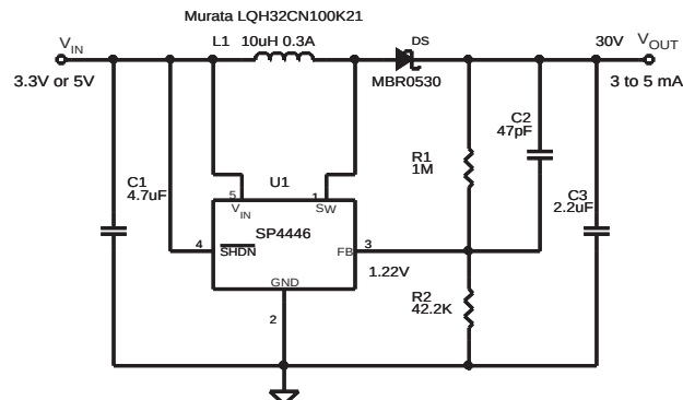
Fig. 2. Pin Diode Driver
