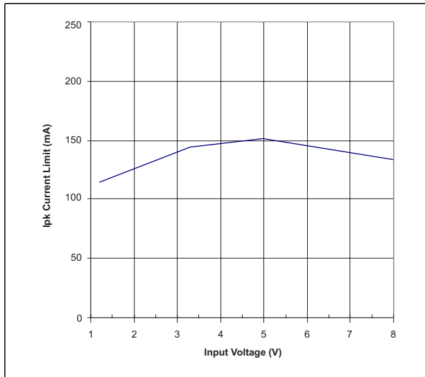
Figure 16. I_{PK} Current Limit vs. V_{IN}
