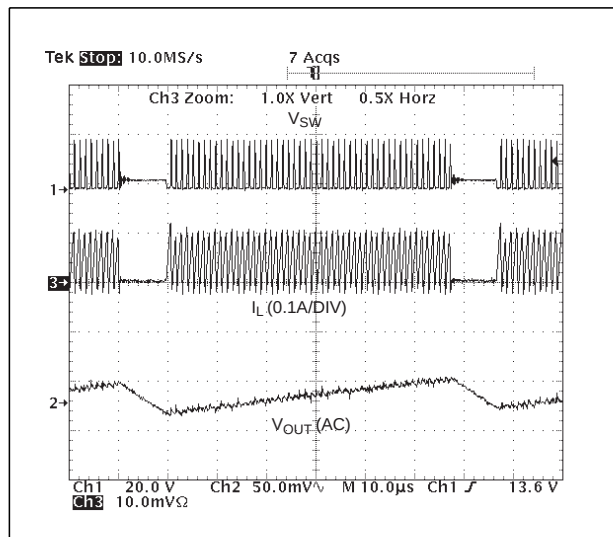
Figure 20. Typical Switching Waveforms ( V_{IN}=3.3\text{V} , V_{OUT}=20\text{V} , I_{OUT}=5\text{mA} )
