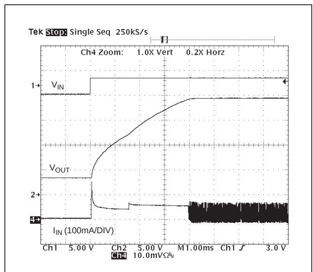
Figure 19. Startup Waveform ( V_{IN}=3.3\text{V} , V_{OUT}=20\text{V} , I_{OUT}=2\text{mA} )
