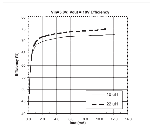
Figure 9. 18V Output Efficiency ( V_{IN}=5\text{V} )
