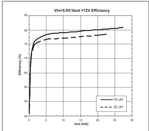
Figure 5. 12V Output Efficiency ( V_{IN}=5\text{V} )
