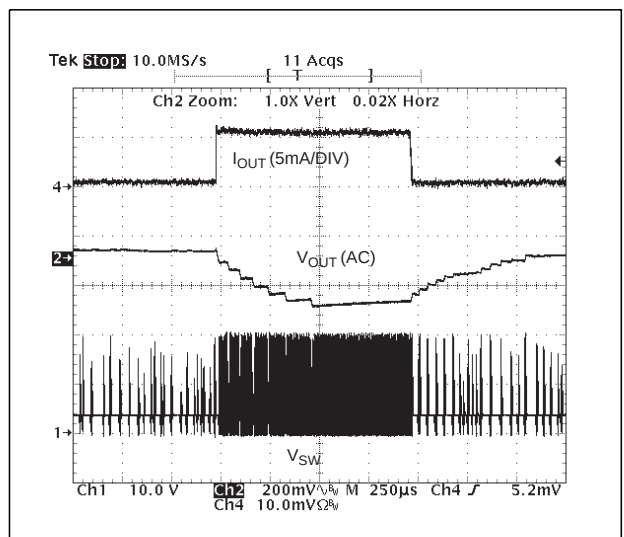
Figure 21. Load Step Transient ( V_{IN}=3.3\text{V} , V_{OUT}=20\text{V} , I_O=100\mu\text{A}\sim 5\text{mA} )
