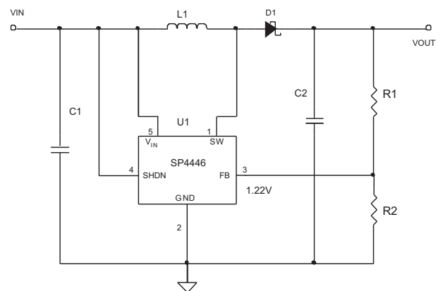
Figure 1. Using SP4446 as Voltage Source
