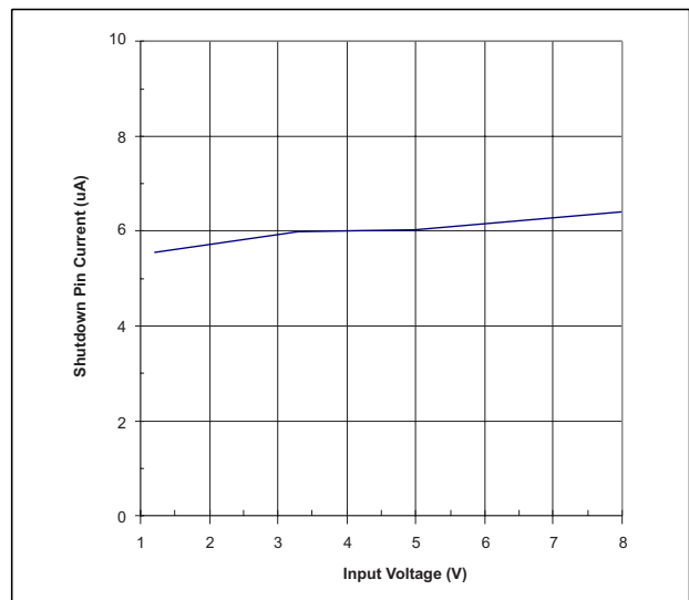
Figure 15. Shutdown Pin Current vs. V_{IN}
