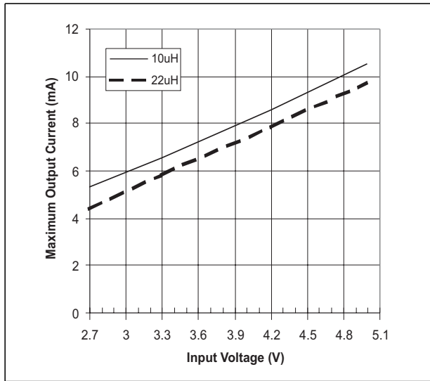
Figure 12. Maximum Output Current vs. V_{IN} ( V_{OUT}=20\text{V} )
