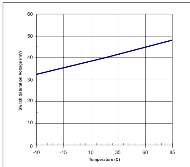
Figure 18. Switch Saturation Voltage V_{CESAT} vs. Temperature ( I_{SW}=50\text{mA} )
