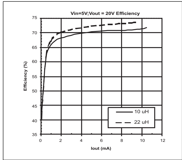
Figure 11. 20V Output Efficiency ( V_{IN}=5\text{V} )
