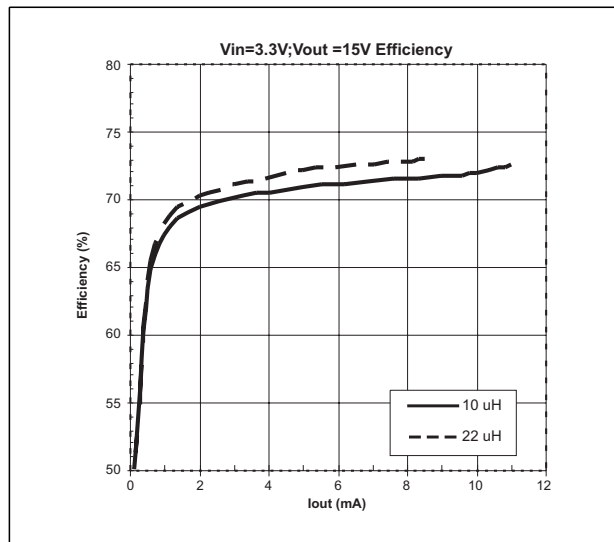
Figure 6. 15V Output Efficiency ( V_{IN}=3.3\text{V} )
