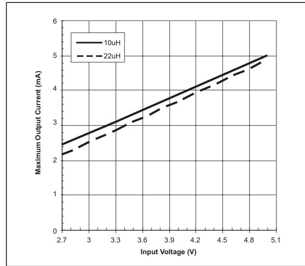
Figure 13. Maximum Output Current vs. V_{IN} ( V_{OUT}=30\text{V} )
