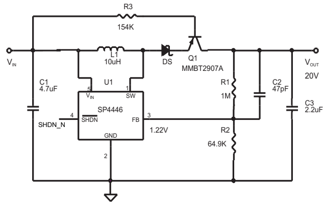
Fig. 3. Load Disconnect in Shutdown
