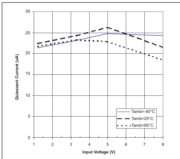
Figure 14. Quiescent Current I_Q vs. V_{IN}
