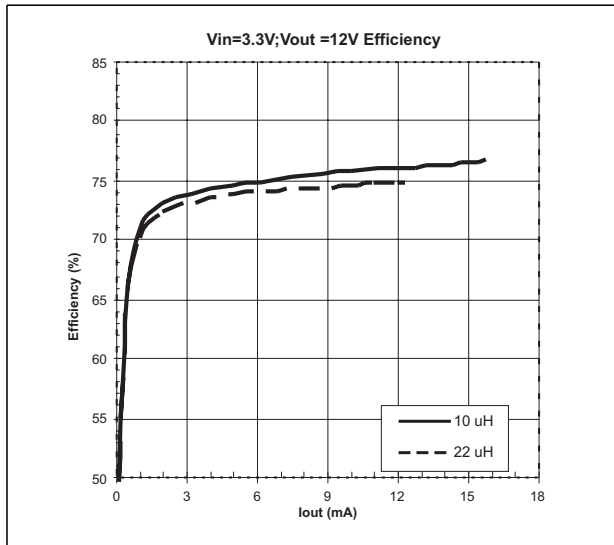
Figure 4. 12V Output Efficiency ( V_{IN}=3.3\text{V} )
