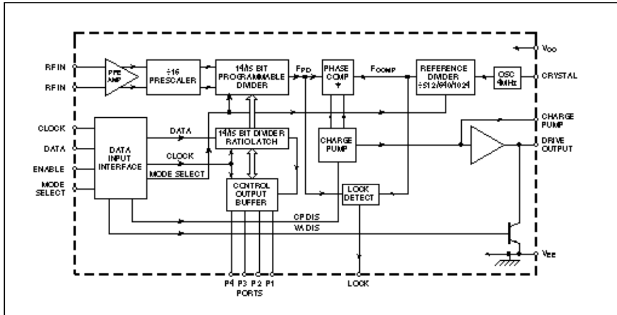
Fig. 3 Block diagram of SP5054
