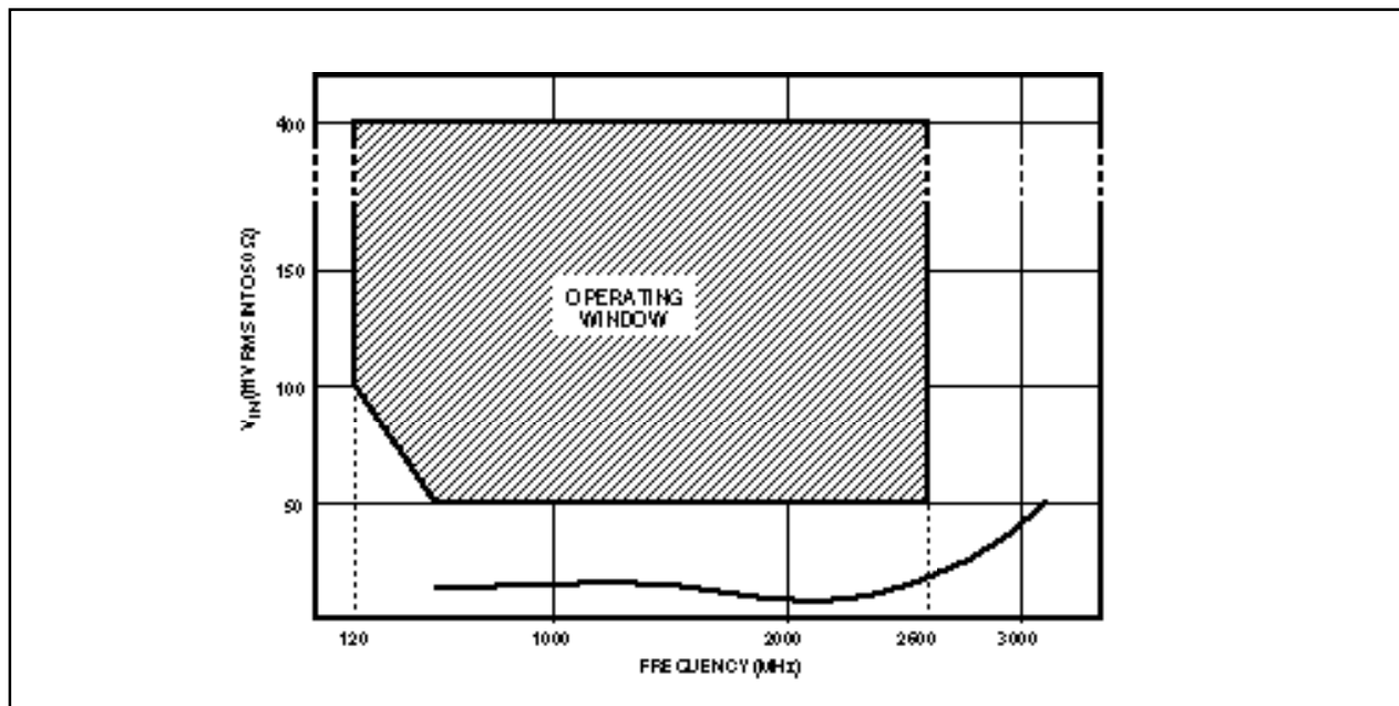
Fig. 6 Typical input sensitivity
