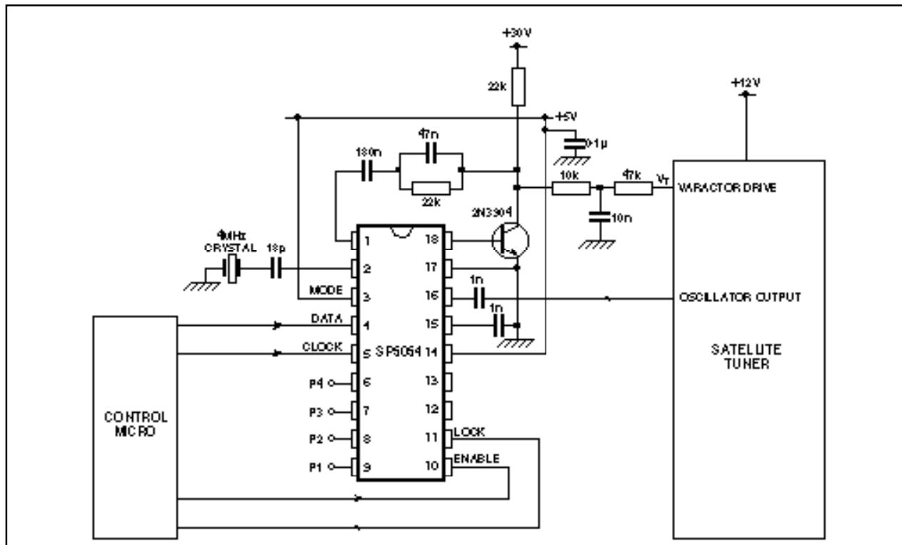
Fig. 5 Typical application ( f_{STEP} = 125kHz )
