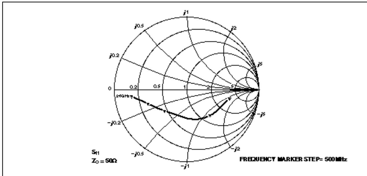
Fig. 2 Typical input impedance
