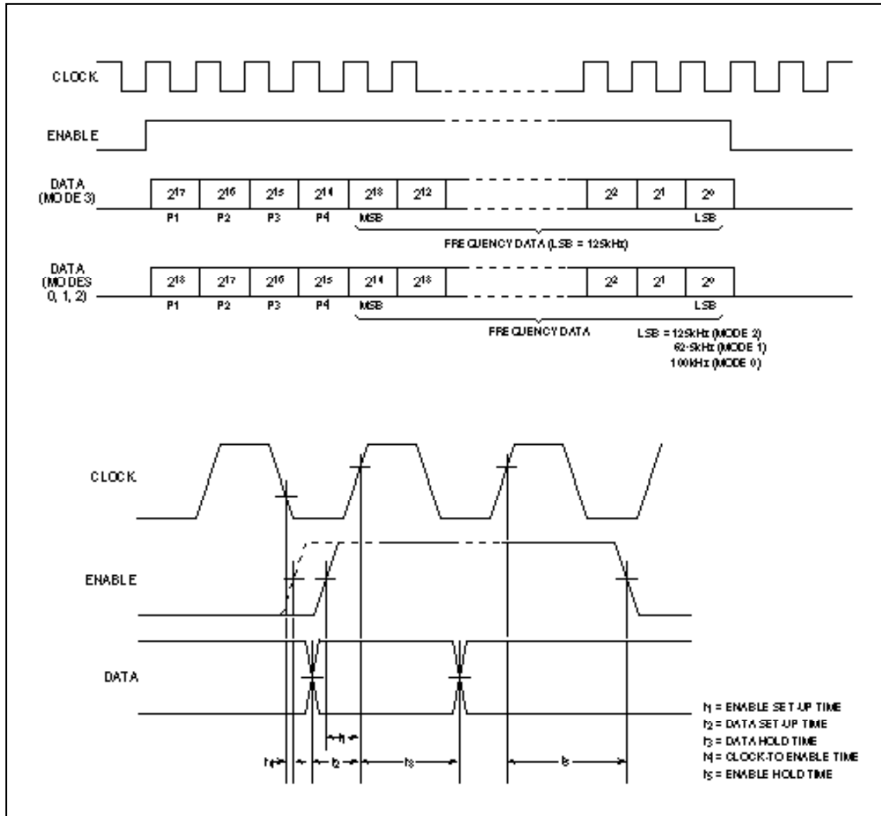
Fig. 4 Data format and timing
