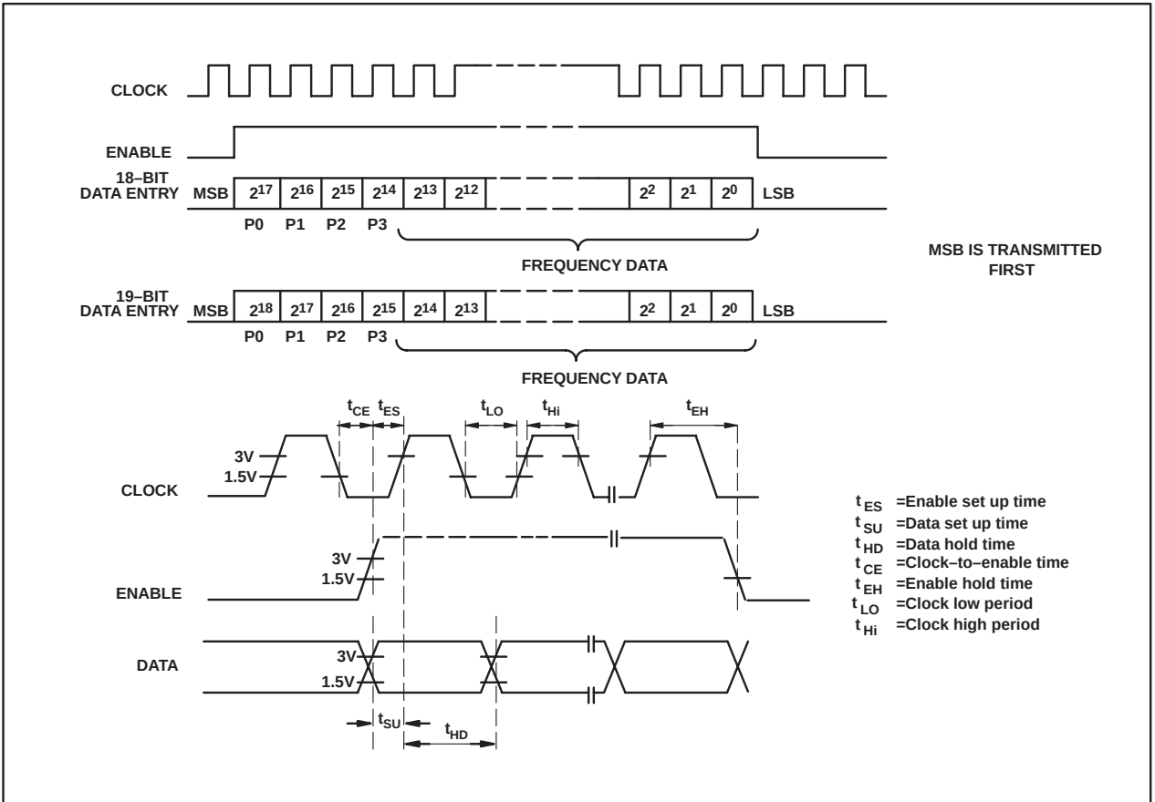
Fig. 4 Data format and timing
