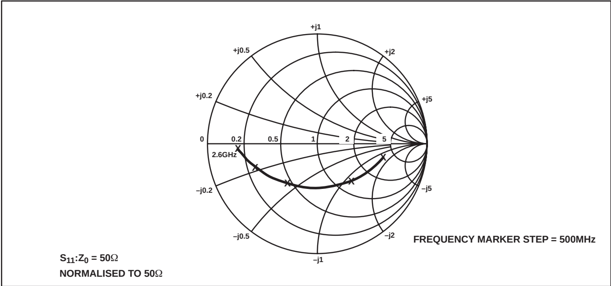
Fig. 2 Typical input impedance
