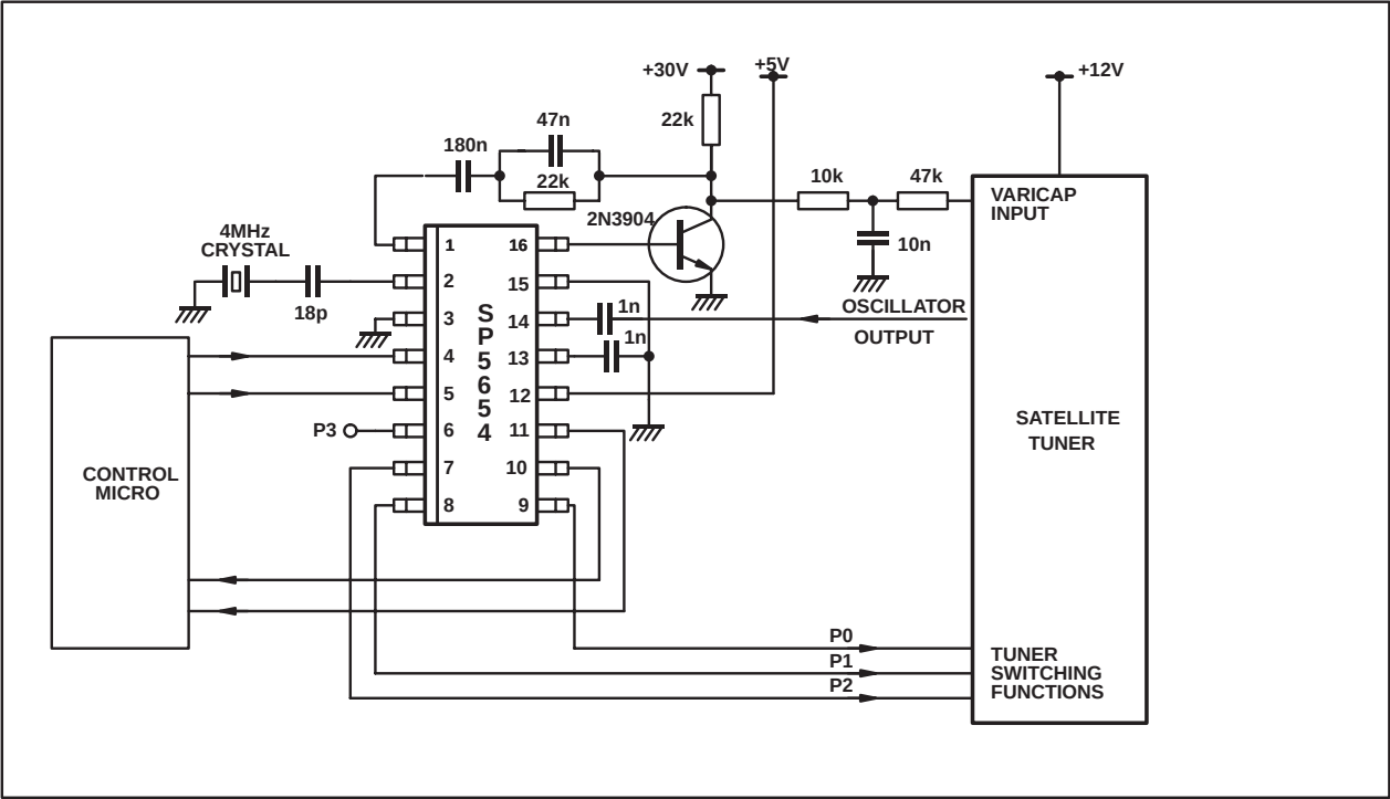
Fig. 5 Typical application (step size = 100kHz)
