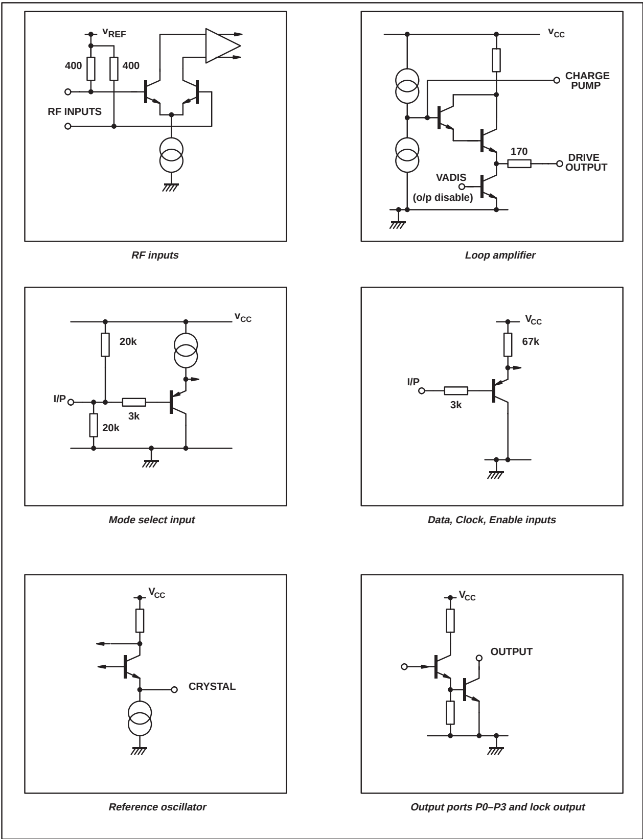
Fig. 7. Input/Output interface circuits
