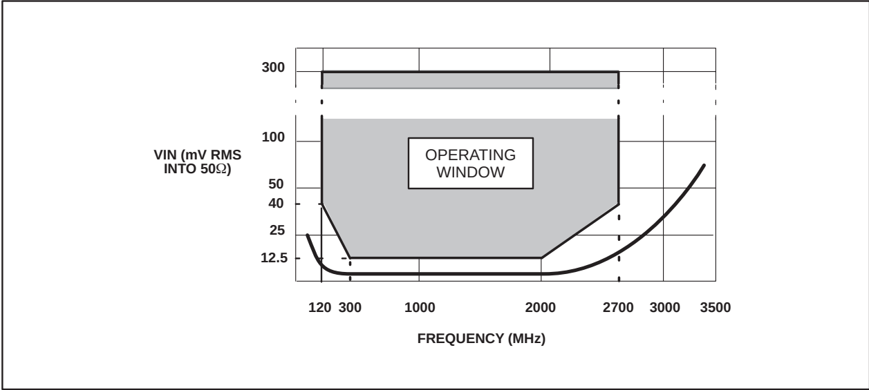
Fig. 6 Typical input sensitivity
