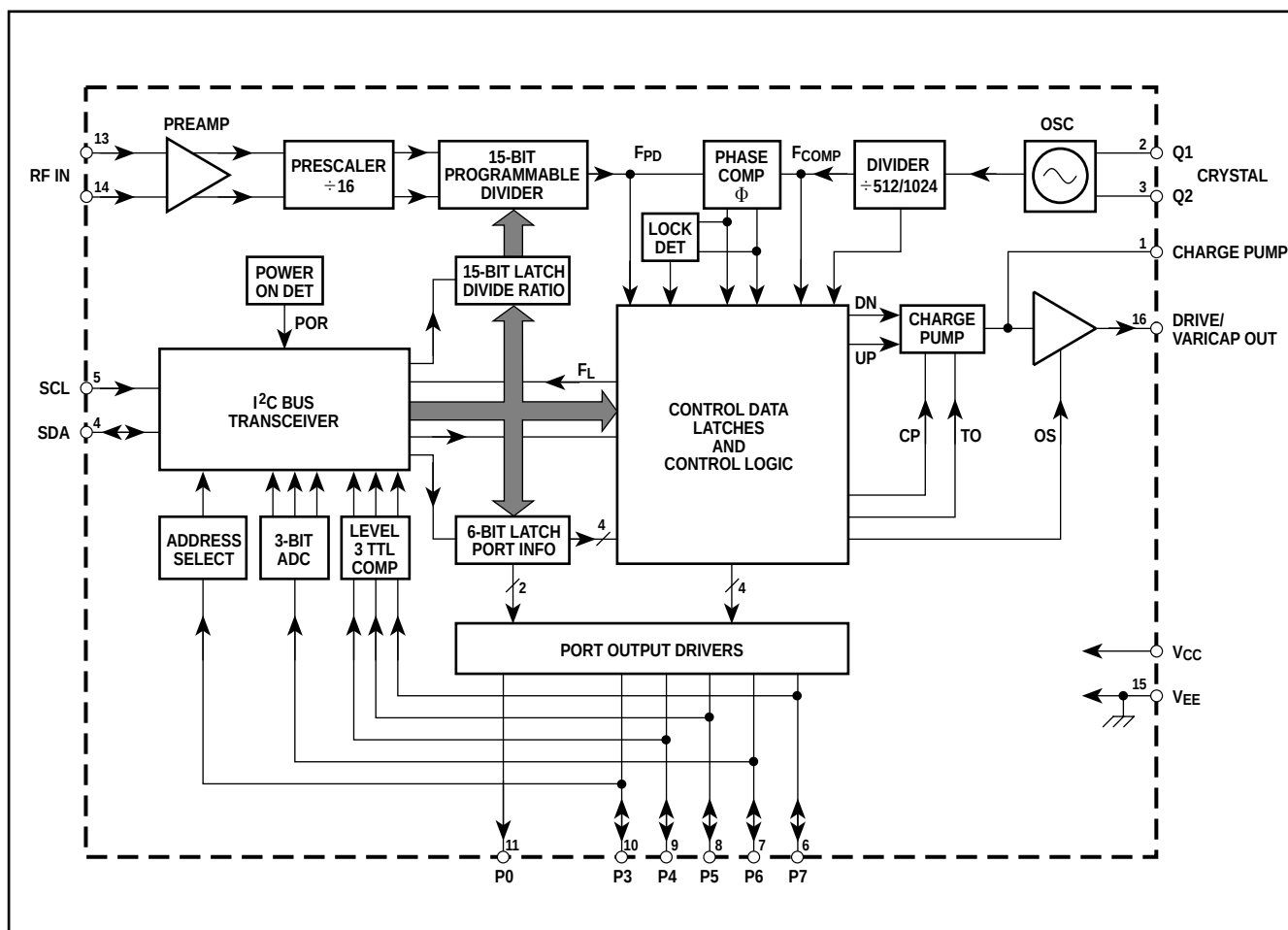
Fig. 2 Block diagram
