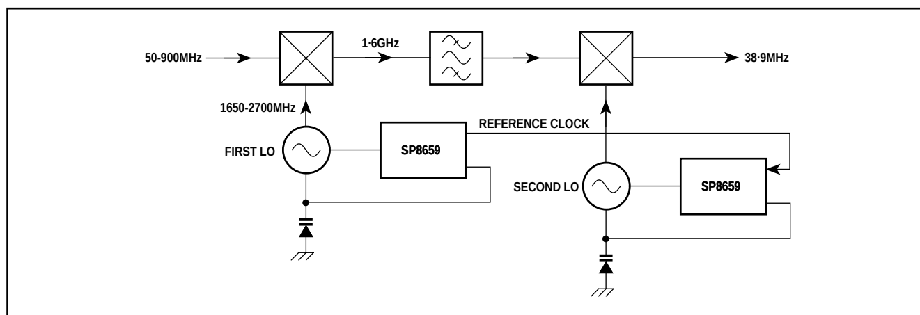
Figure 5 - Example of double conversion from VHF/UHF frequencies to TV IF
