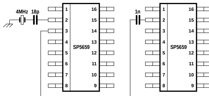
Figure 9 - Two SP5659 devices using a common reference
