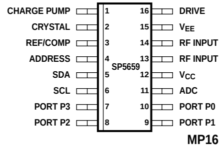
Figure 1 – Pin connections – top view
