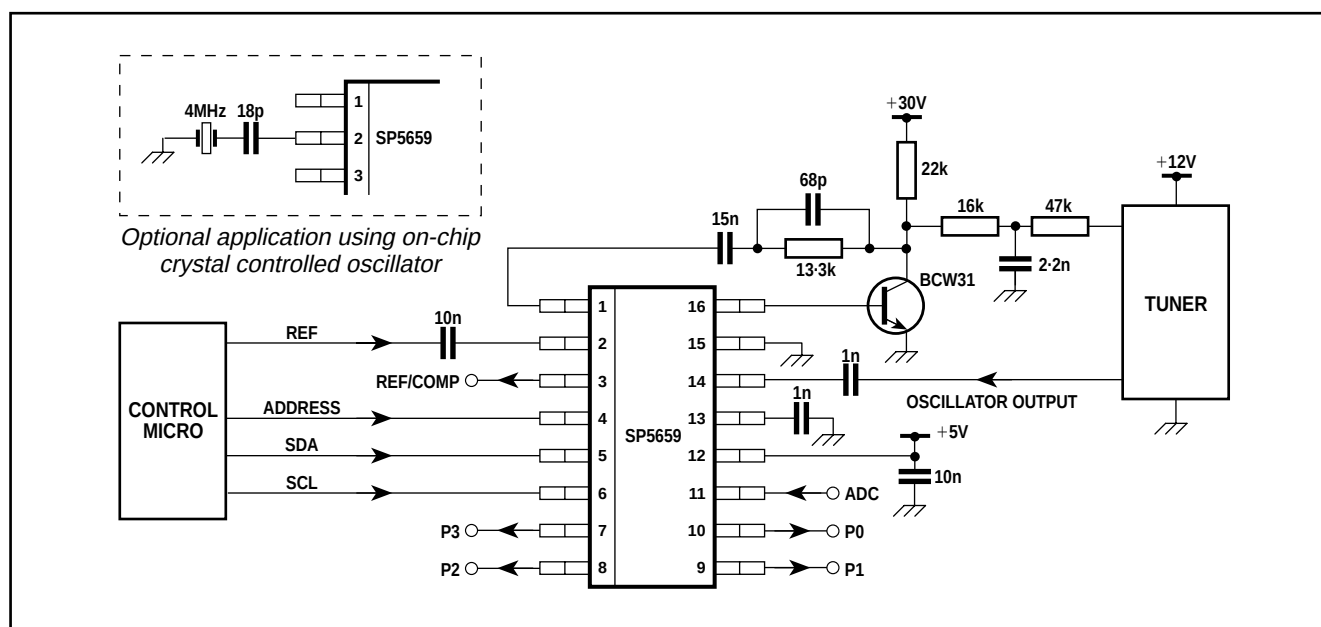
Figure 6 - Typical application
