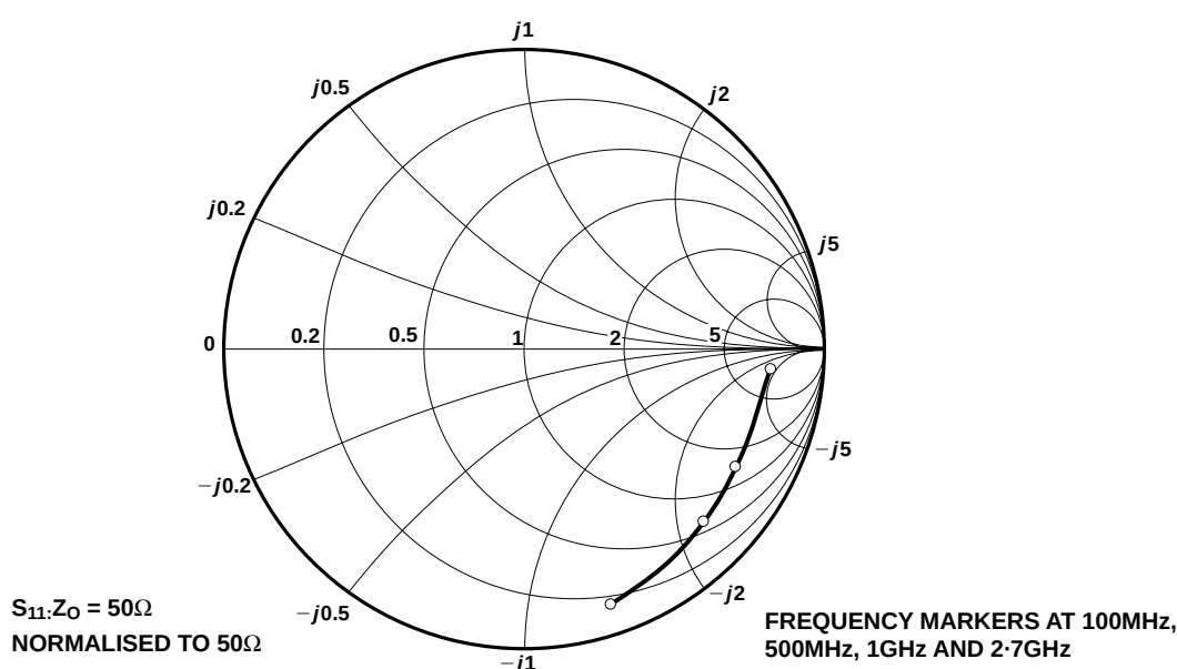
Figure 10 - Typical RF input impedance
