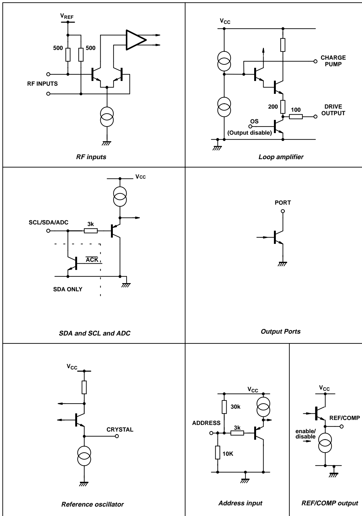
Fig. 14 Input/Output interface circuits
