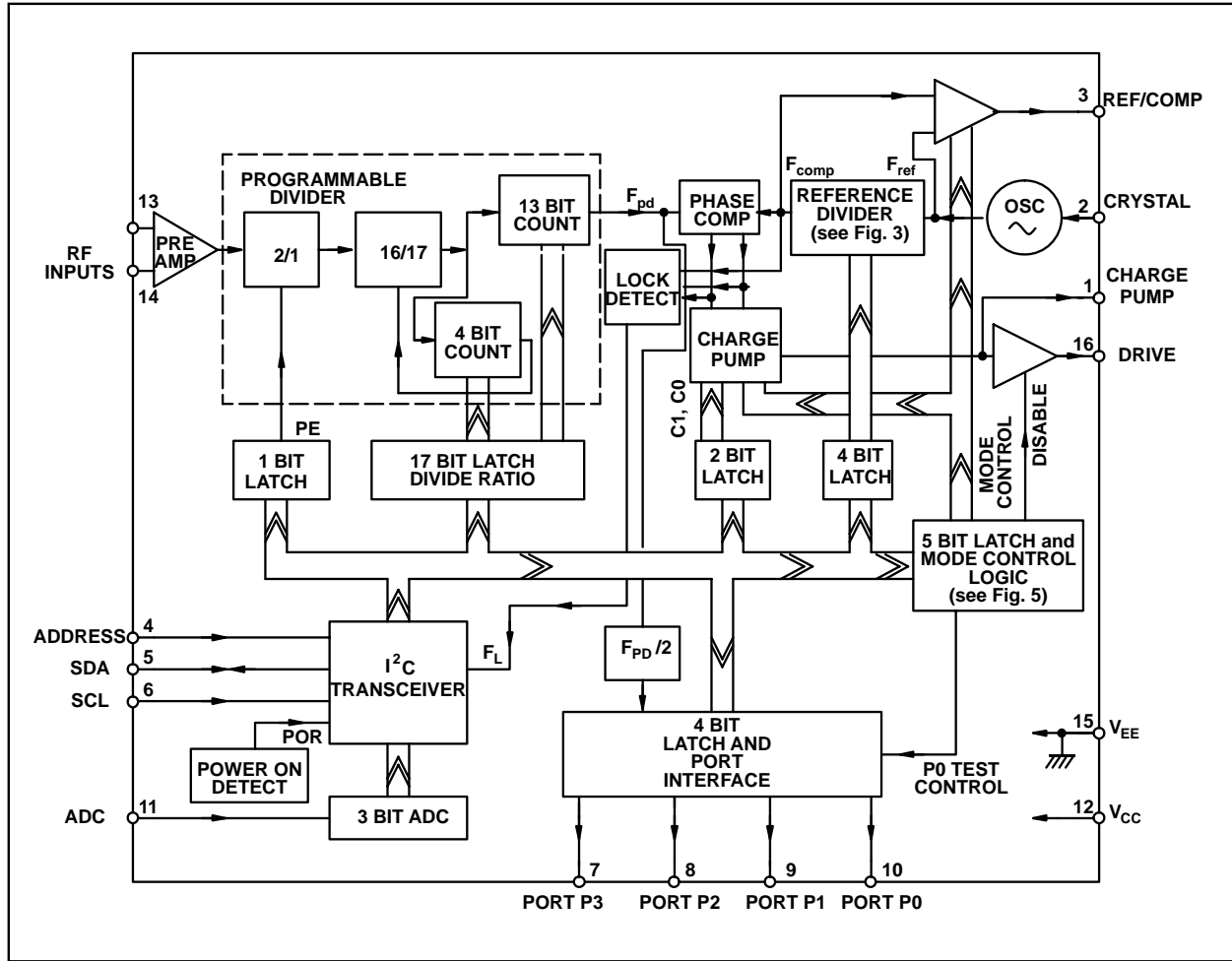
Fig. 2 Block diagram
