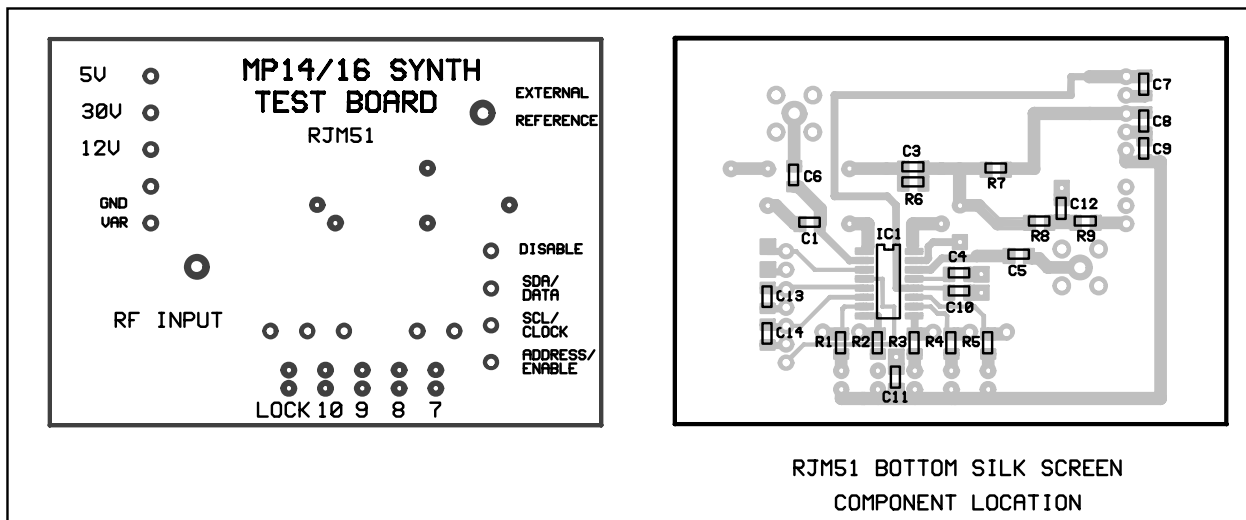
Fig. 11 Test board (layout)
