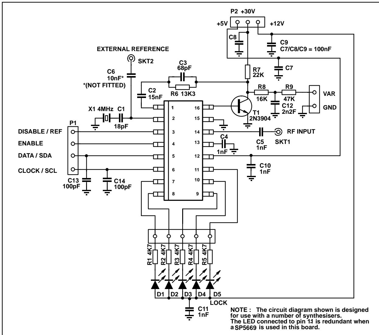
Fig. 10 Test board
