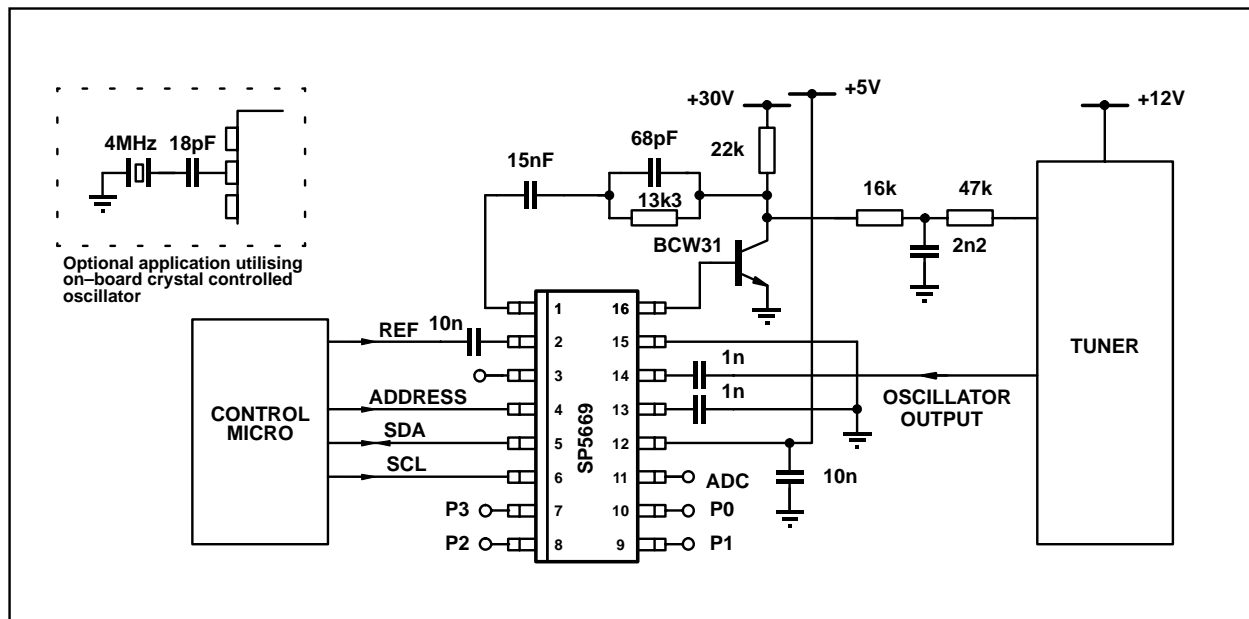
Fig. 9 Typical application
