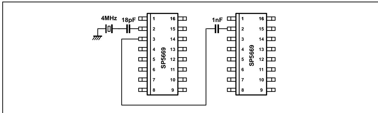
Fig. 12 Driving two devices from a common reference
