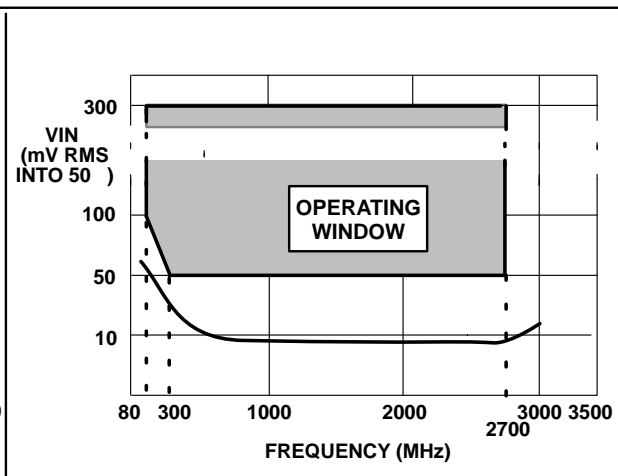
Fig. 7b Typical input sensitivity (prescaler disabled, PE=1)
