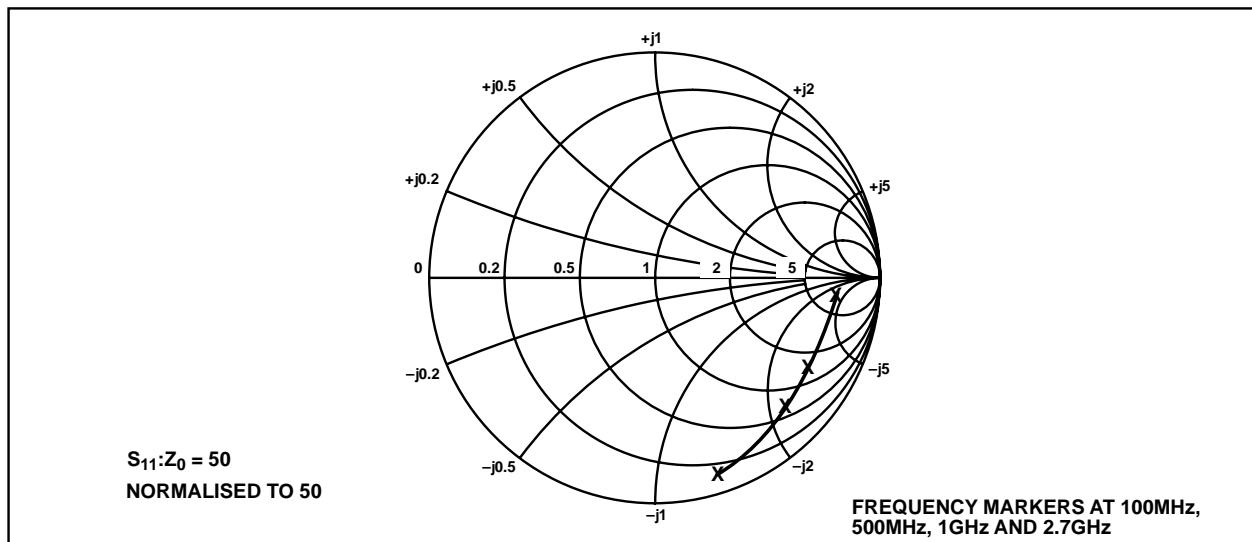
Fig. 13 typical RF input impedance
