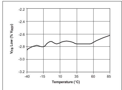
Figure 13. V_{FB} 3% Low Comparator vs. Temperature
