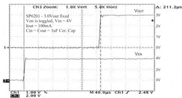
Fig. 23: Turn on time, I_O=100\text{mA} , 4V_{IN}
