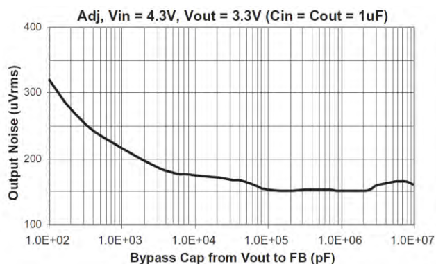
Fig. 42: Noise Performance 10Hz to 100kHz
