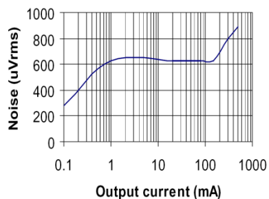
Fig. 20: Output Noise, C_{BYP} = \text{open}
