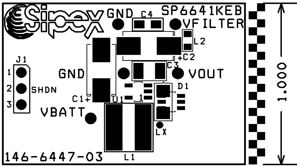
FIGURE 4: SP6641A/6641B COMPONENT PLACEMENT
