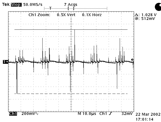
Figure 1. SP6641B Switching Signals on 330uF: V_{in} = 2.0V, I_{out} = 300mA, Spikes = 1.0Vpp
