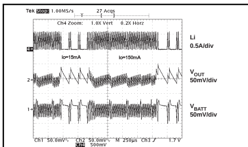
Figure 22. Load Transient Response, V_{batt}=1.3\text{V} , ( V_{out}=3.3\text{V} ), R_{lim}=2.5\text{k} , L_i=22\mu\text{H} Sumida CD-43
