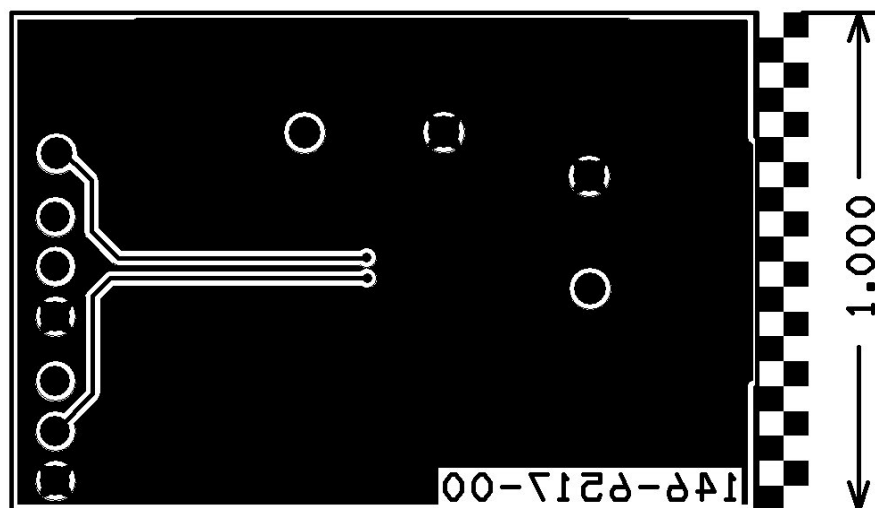
FIGURE 5: SP6655ER PC LAYOUT BOTTOM SIDE
