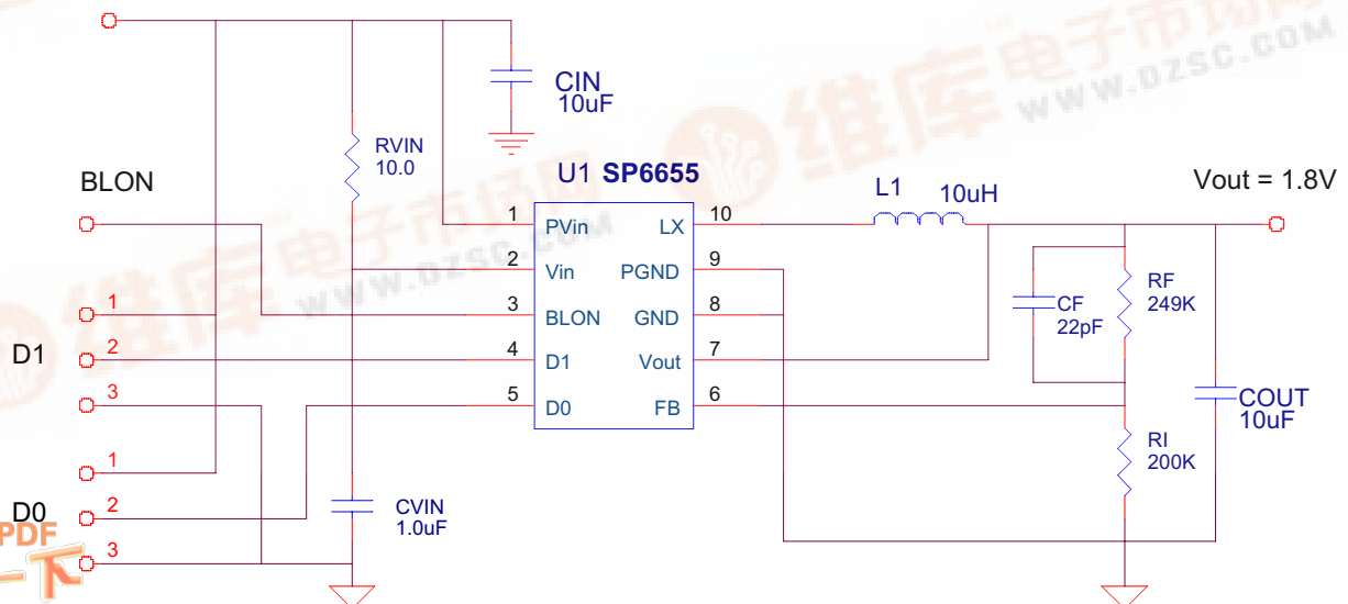
FIGURE 1. SP6655 1.8V OUTPUT EVALUATION BOARD SCHEMATIC
