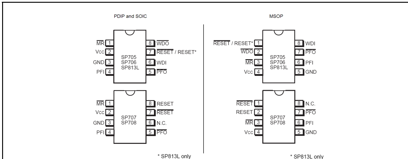
Fig. 3: Pin Assignment
