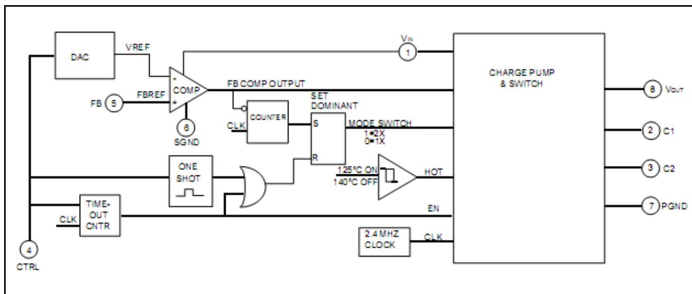
Fig. 2: SP7686 Block Diagram
