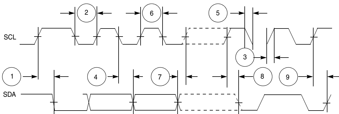
Figure 38. I²C input/output timing
