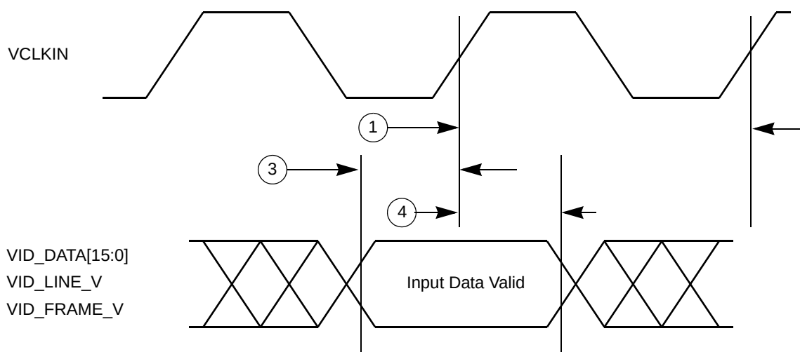
Figure 33. Video interface timing
