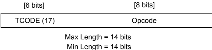
Figure 24-56. Read Register Message
