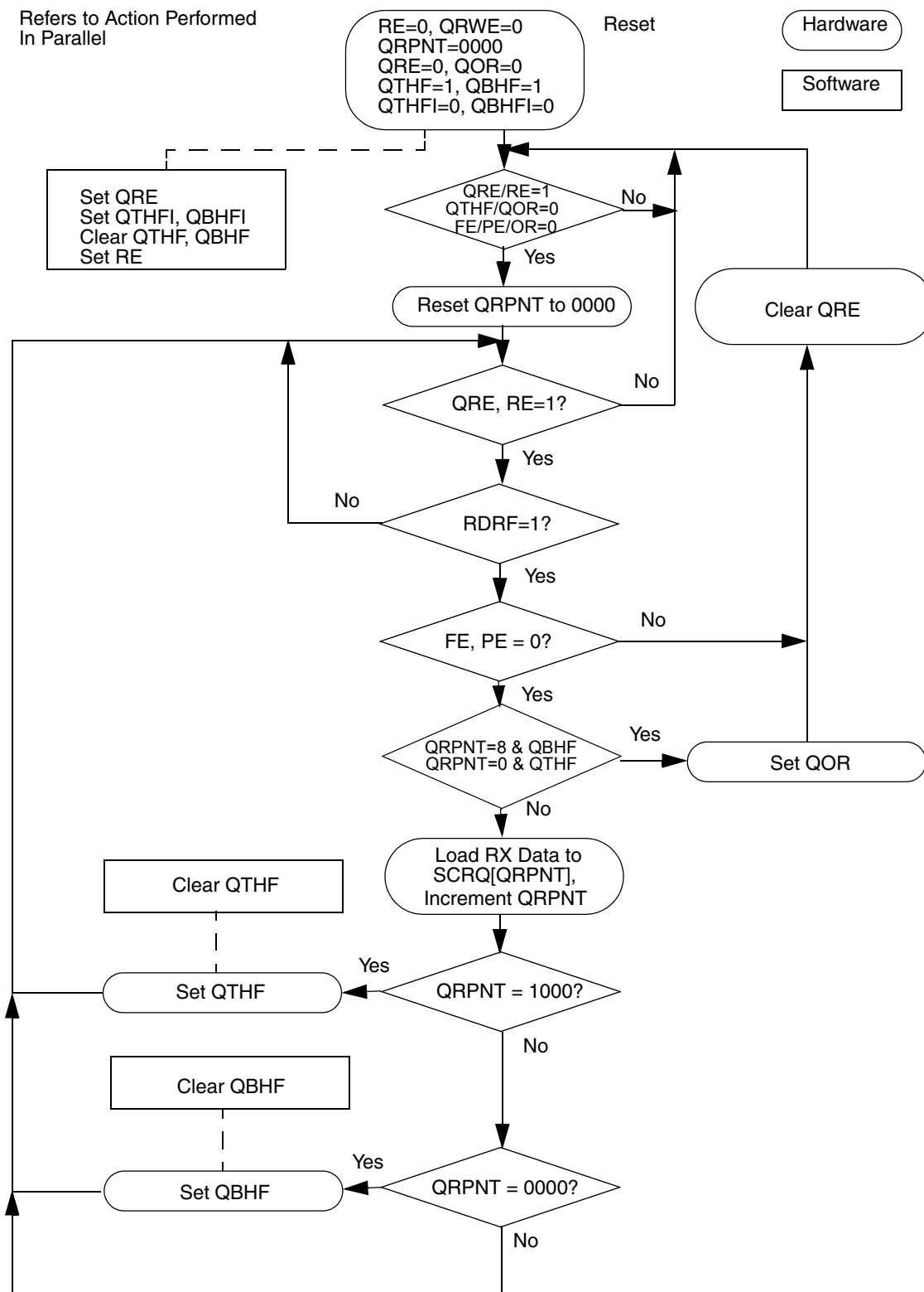
Figure 15-39. Queue Receive Flow
