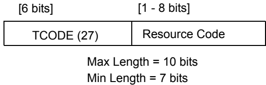
Figure 24-32. Program Trace Full Message Format
