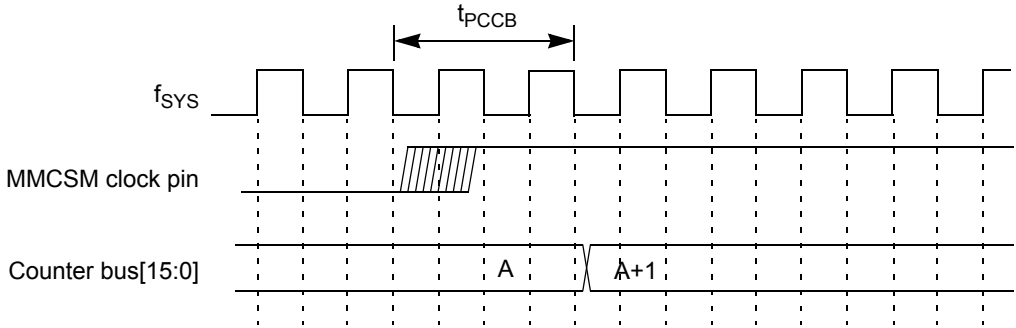
Figure F-53. MMCSM Clock Pin To Counter Bus Increment Timing Diagram
