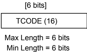
Figure 24-55. Target Ready Message
