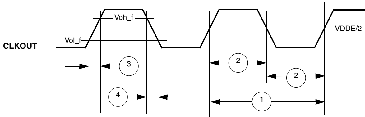
Figure 16. CLKOUT timing
