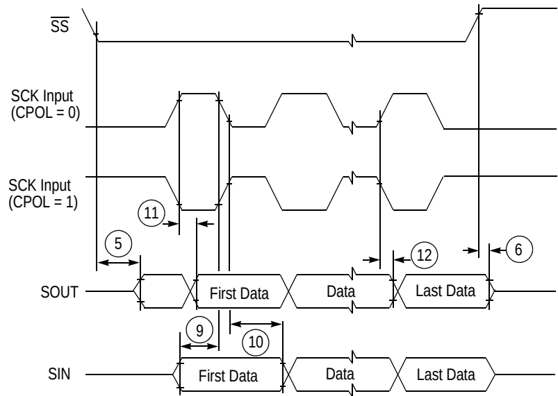
Figure 19. DSPI Classic SPI Timing — Slave, CPHA = 1
