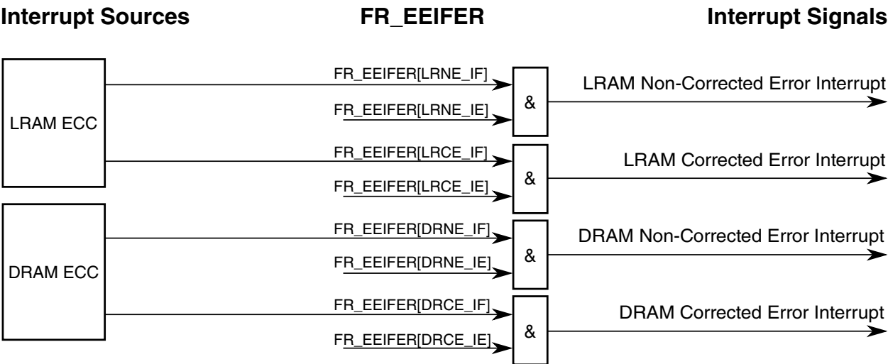
Figure 50-34. Scheme of FR_EEIFER interrupt signal generation
