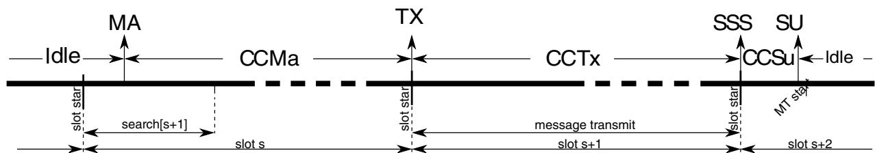
Figure 50-10. Message Transmission Timing
