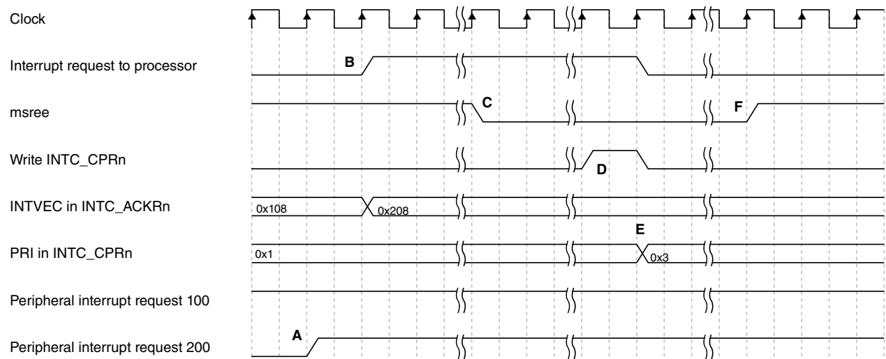
Figure 21-6. Timing diagram of raised priority preserved
