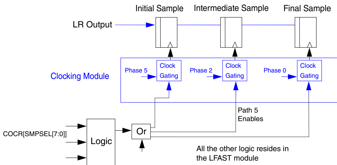
Figure 48-11. Sampler 5 Logic
