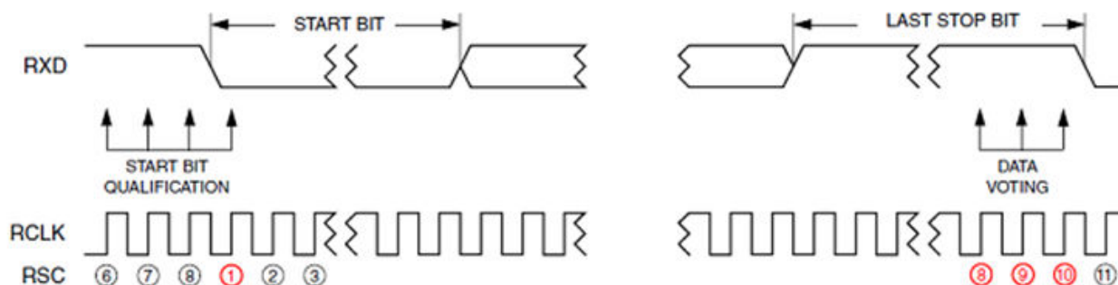
Figure 52-62. Slower receiver
