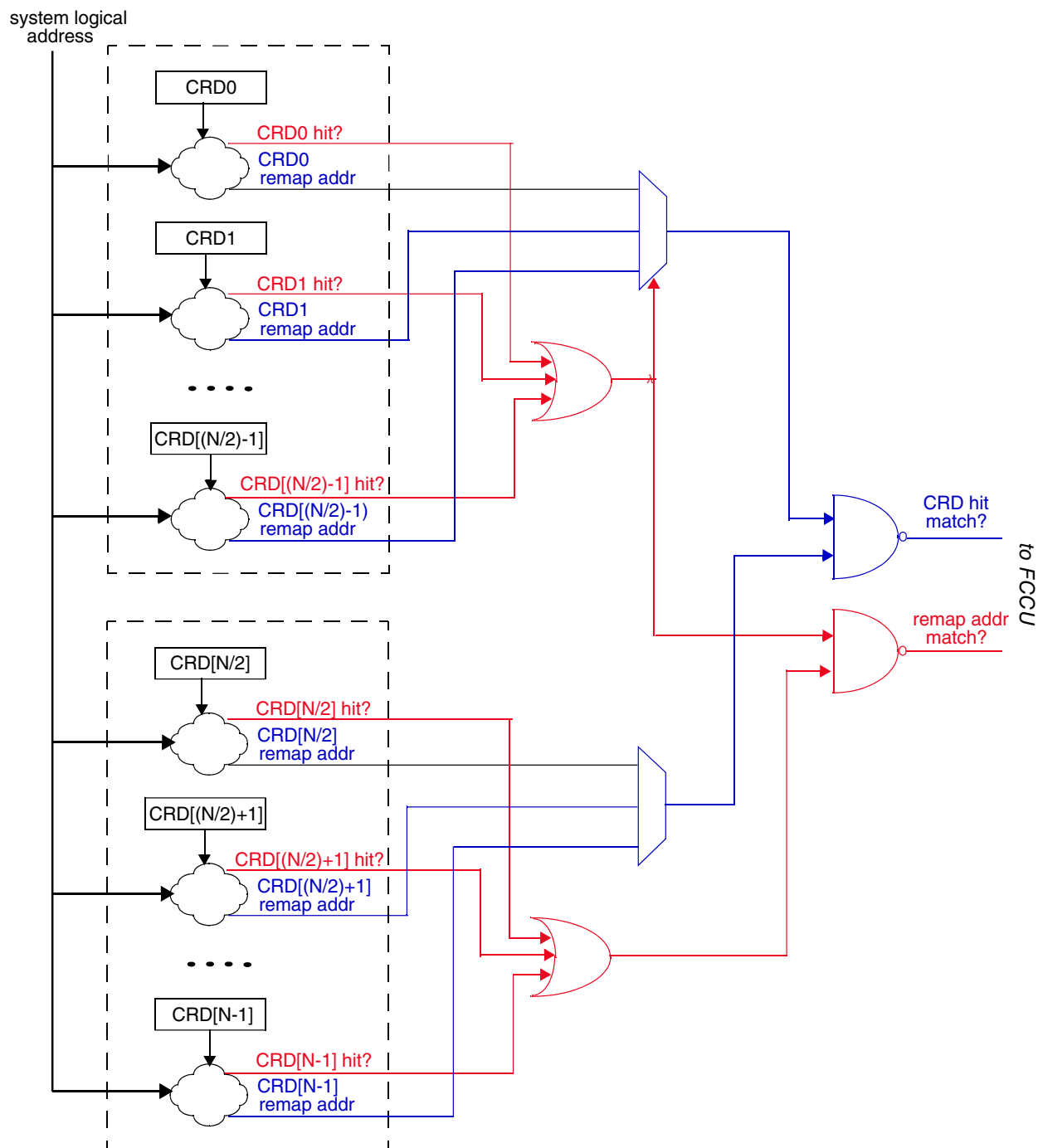
Figure 31-3. Safety-critical calibration remap datapath with redundancy
