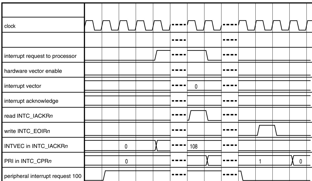
Figure 21-3. Timing diagram of software vector mode handshaking
