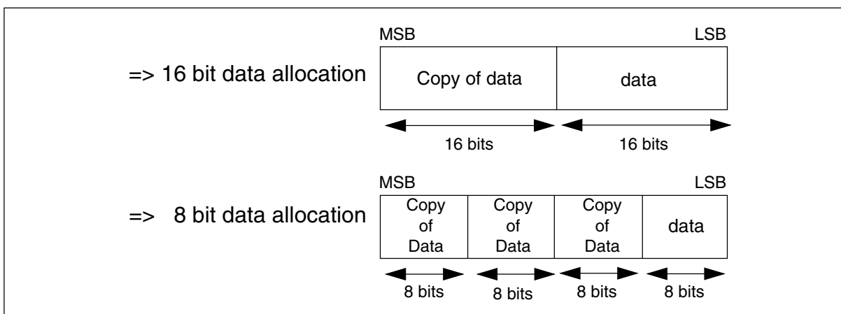
Figure 47-13. Data allocation
