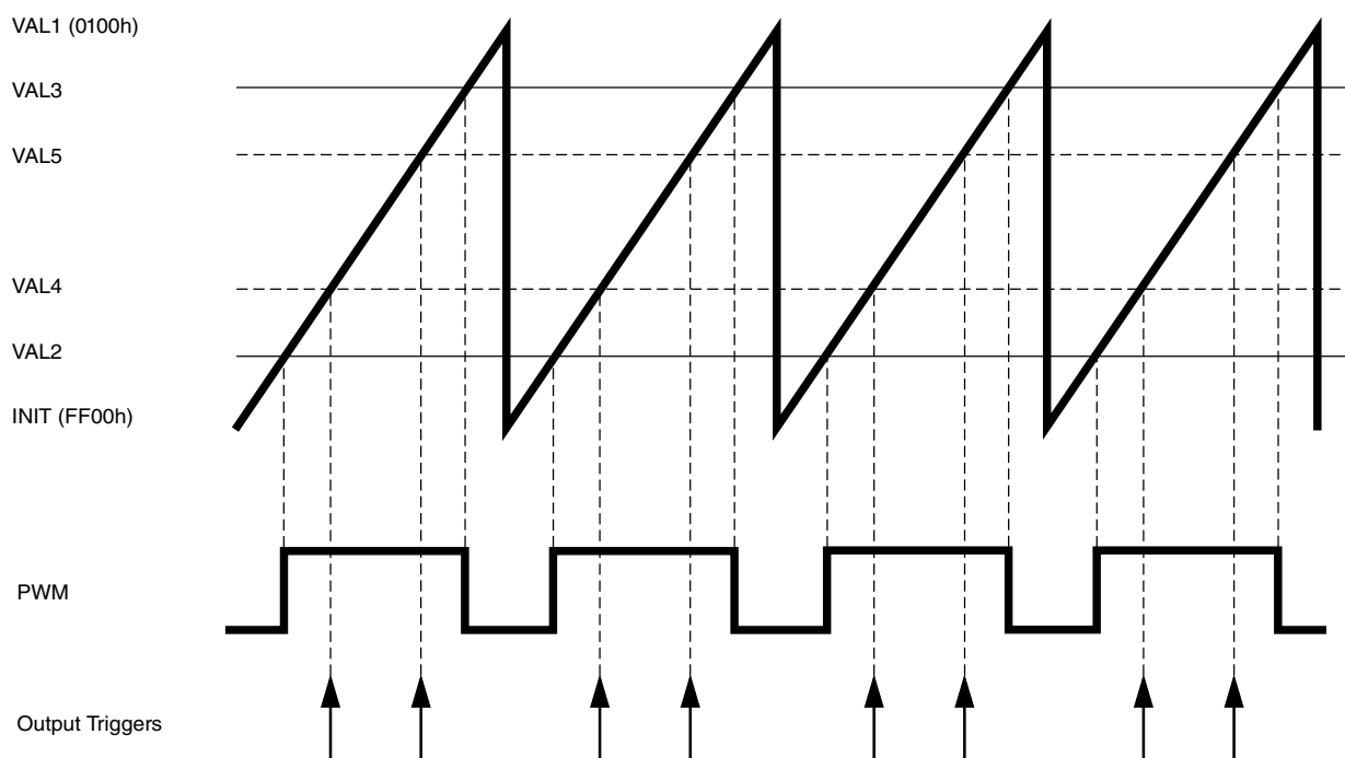
Figure 40-8. Multiple Output Trigger Generation in Hardware
