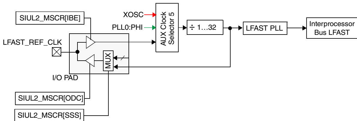
Figure 13-4. Device LFAST SysClk
