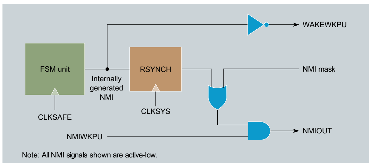
Figure 69-6. NMI/WKPU scheme
