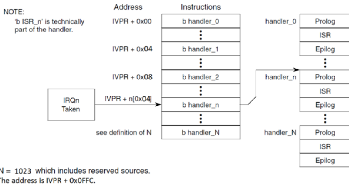
Figure 7-4. Hardware vector mode: program flow
