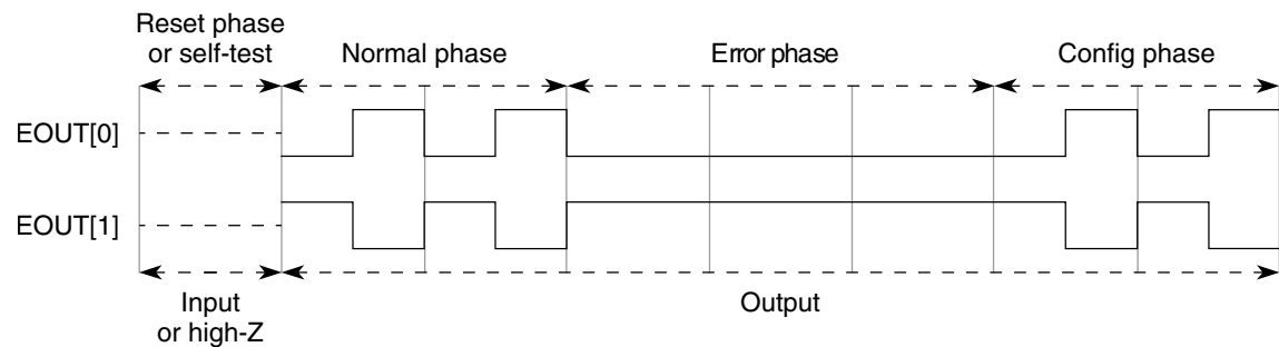
Figure 69-12. Time-switching protocol
