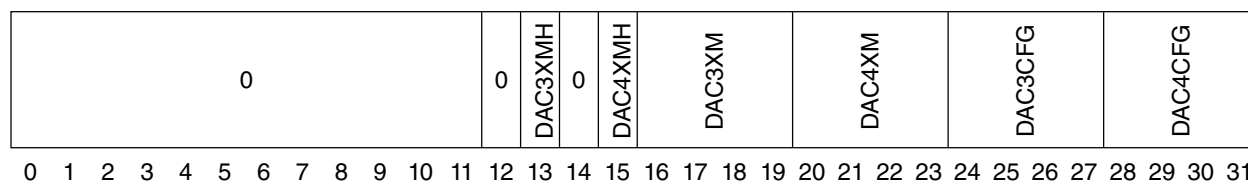
Figure 60-9. DBCR7 Register
