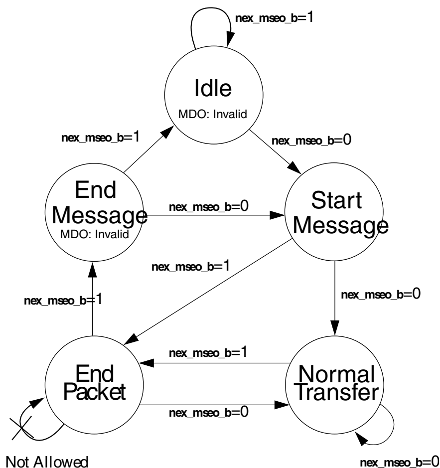
Figure 62-54. Single pin MSEO transfers
