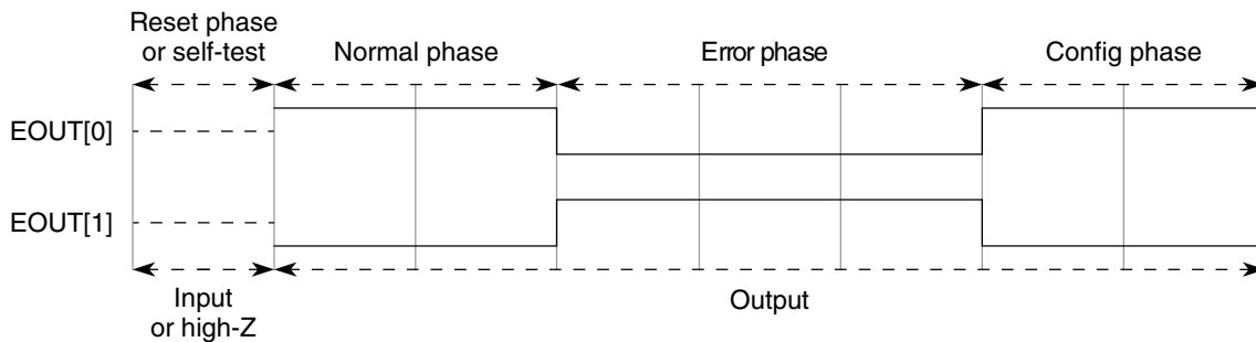
Figure 69-13. Bi-stable protocol
