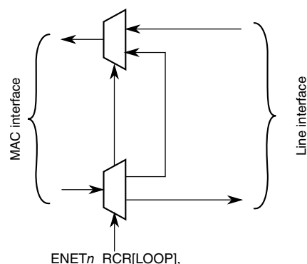
Figure 53-13. Loopback options
