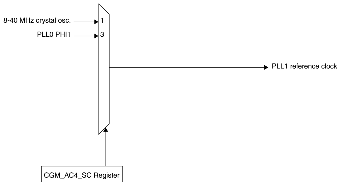
Figure 27-9. MC_CGM Auxiliary Clock 4 Generation Overview
