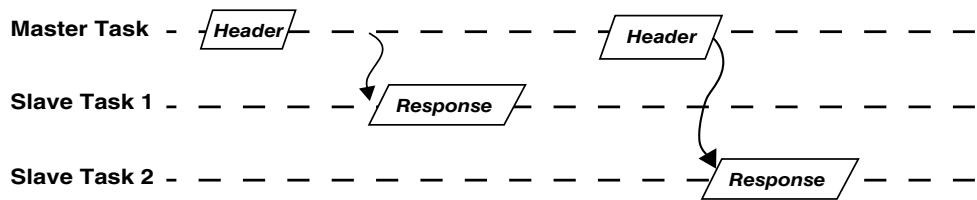
Figure 52-2. Frames
