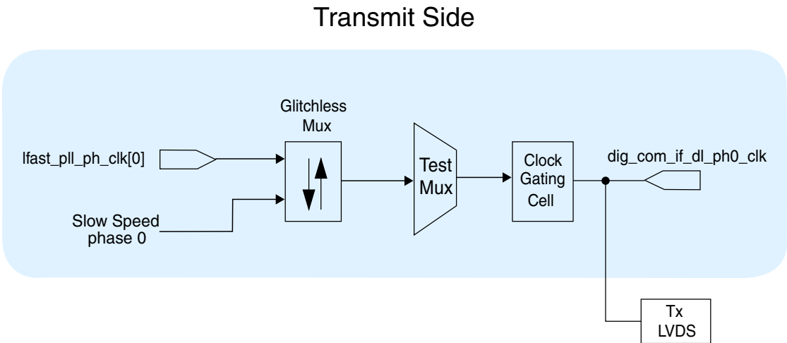
Figure 48-28. Transmit Clocks Muxing
