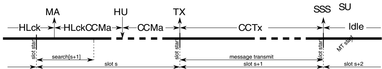
Figure 50-11. Message Transmission from HLck state with unlock
