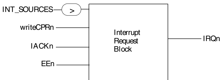
Figure 21-5. Interrupt Request Block Diagram
