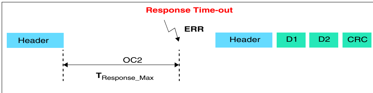
Figure 52-11. No response
