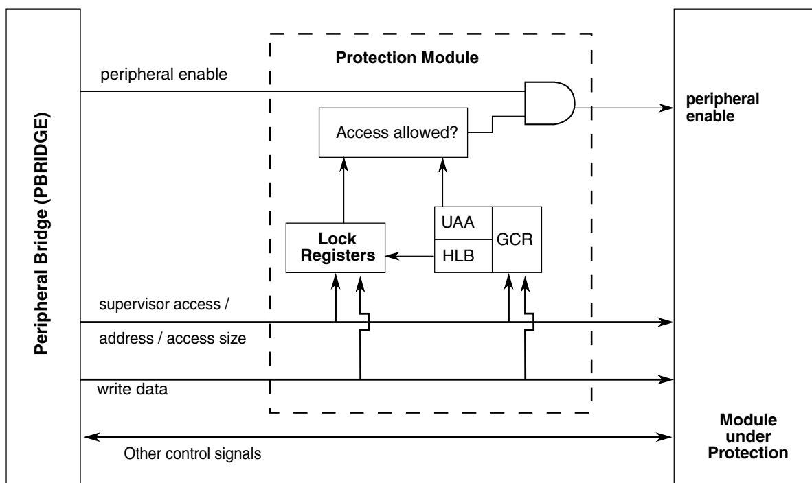
Figure 71-1. REG_PROT Block Diagram
