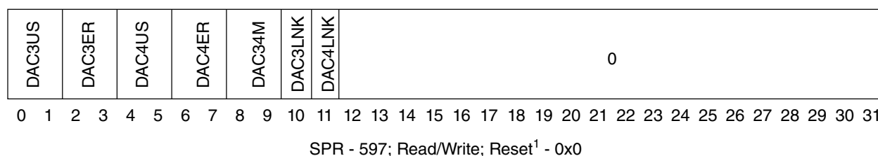
Figure 60-10. DBCR8 Register
