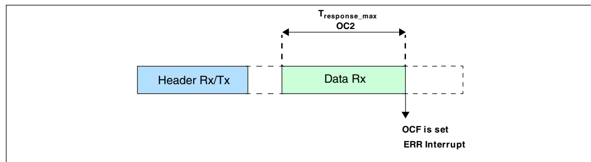
Figure 52-56. Response timeout
