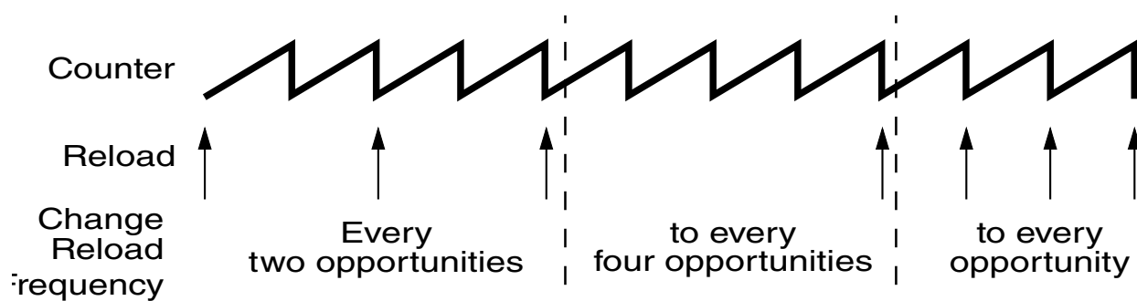
Figure 40-31. Full Cycle Reload Frequency Change
