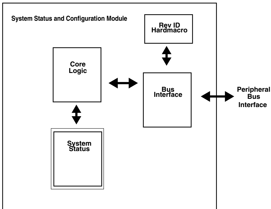
Figure 56-1. SSCM block diagram
