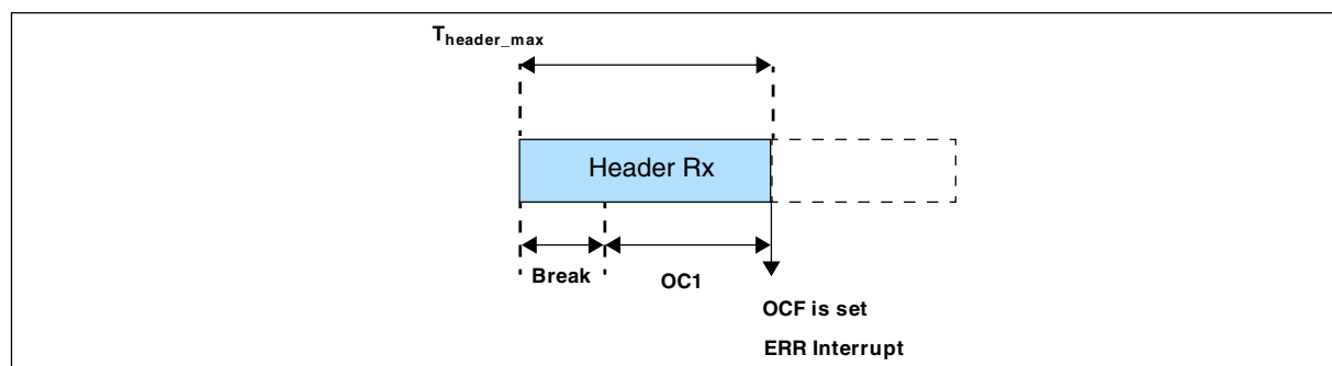
Figure 52-58. Header timeout
