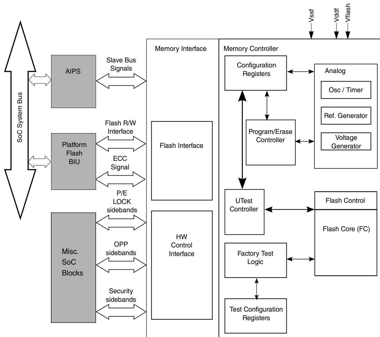
Figure 32-1. c55fmc block diagram
