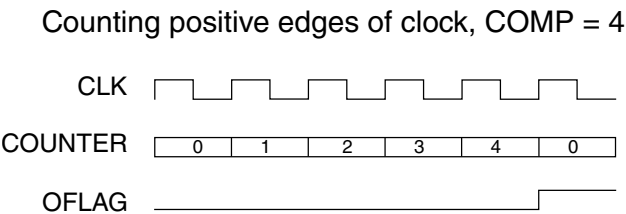
Figure 39-11. OFLAG timing during continuous counting
