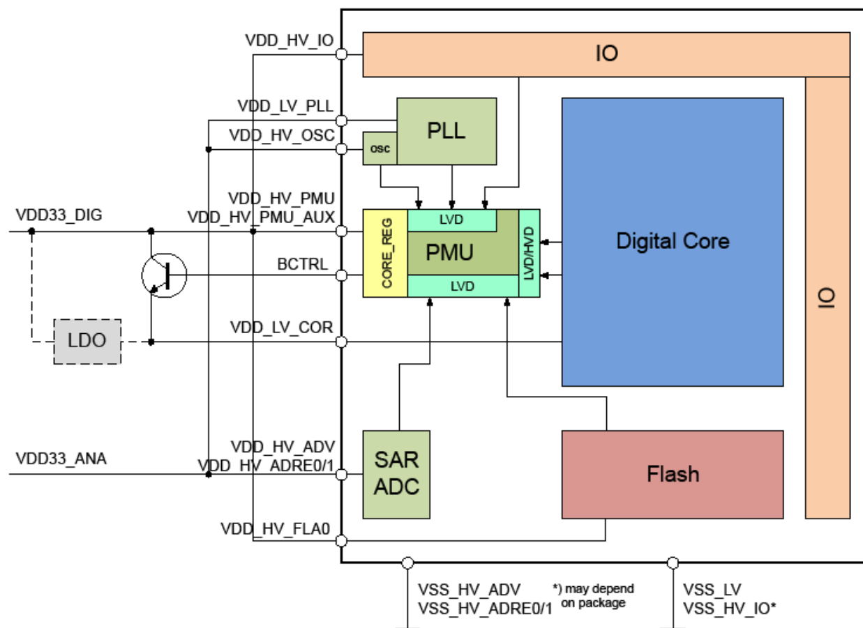
Figure 12-2. Supply concept
