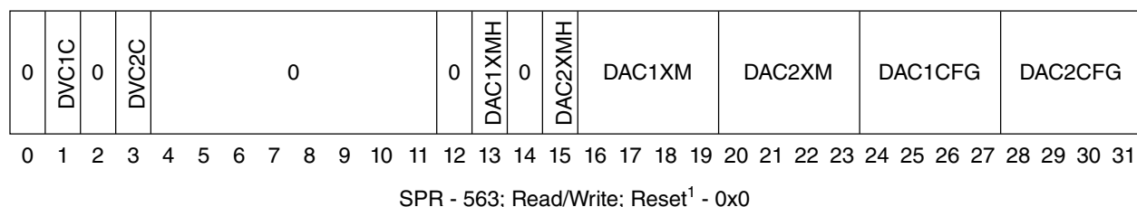
Figure 60-6. DBCR4 Register
