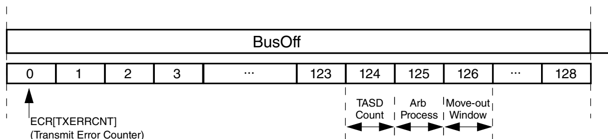
Figure 45-6. Arbitration at the end of bus off and move-out time windows
