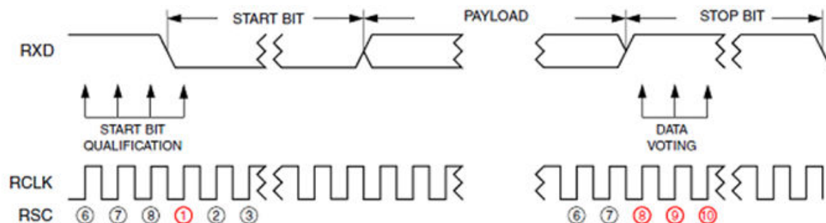
Figure 52-61. Faster receiver
