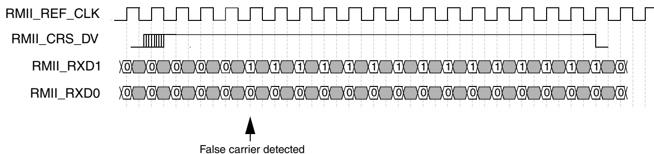
Figure 53-20. RMI receive operation with false carrier
