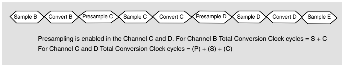
Figure 36-5. Presampling sequence
