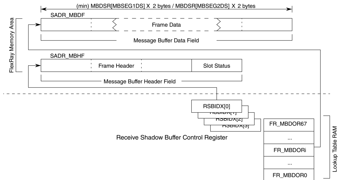
Figure 50-4. Receive Shadow Buffer Structure
