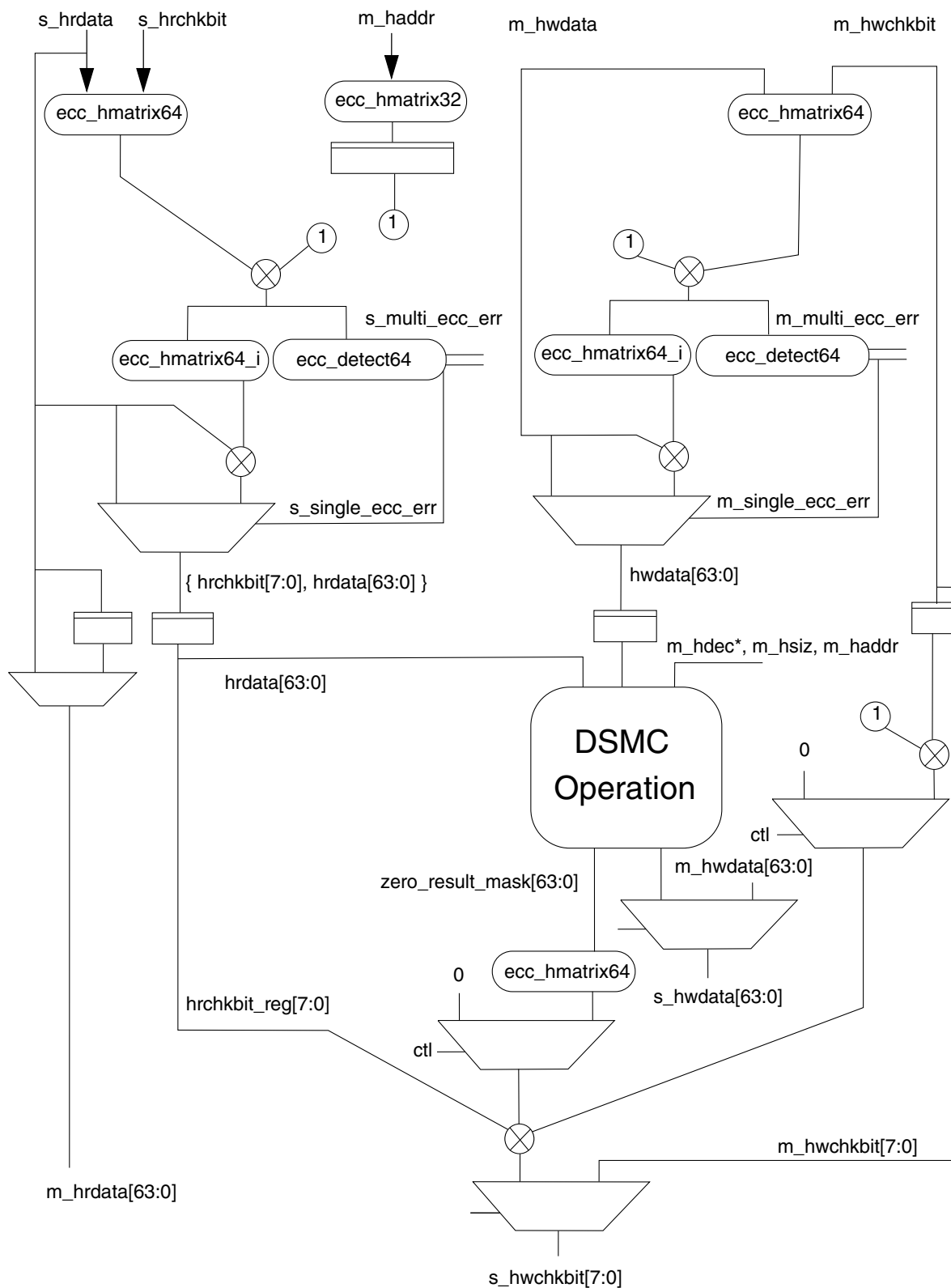
Figure 34-1. DSMC Block diagram
