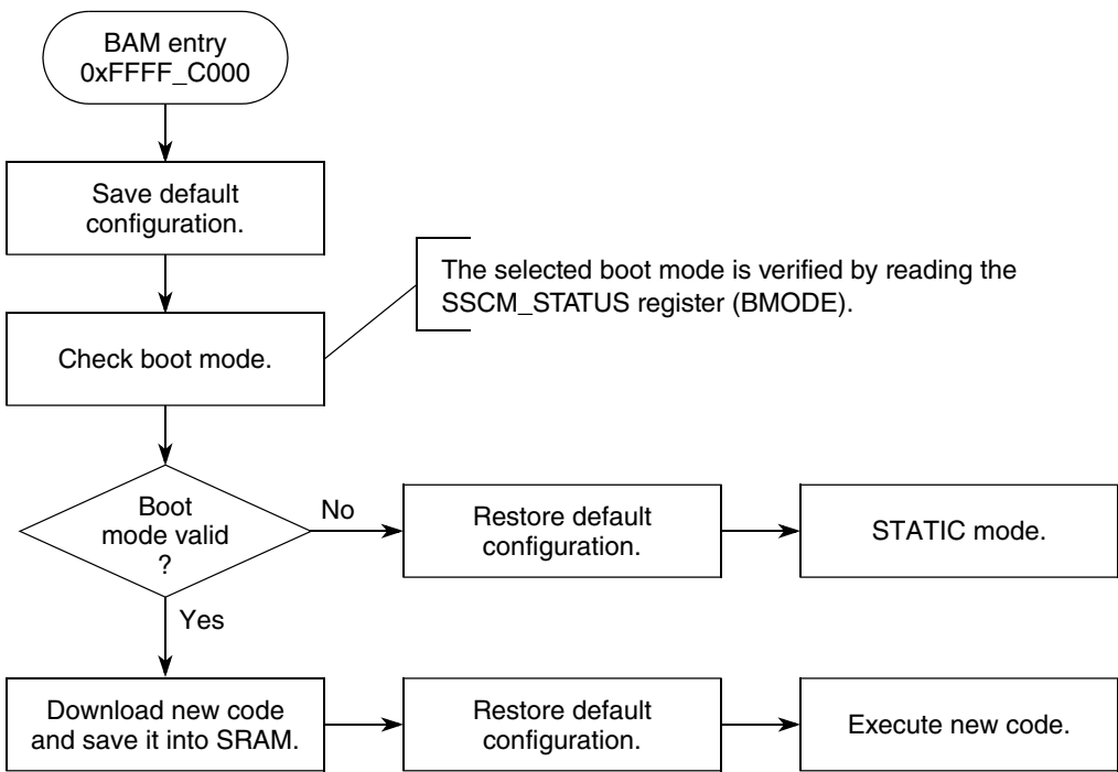
Figure 55-2. BAM logic flow
