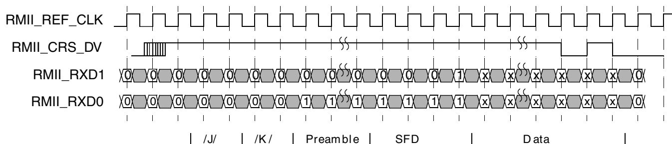
Figure 53-19. RMII receive operation
