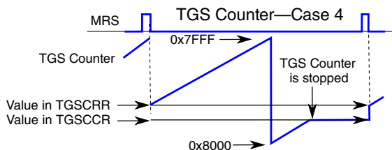
Figure 41-7. TGS counter behavior
