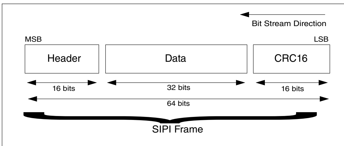
Figure 47-12. Read answer transfer
