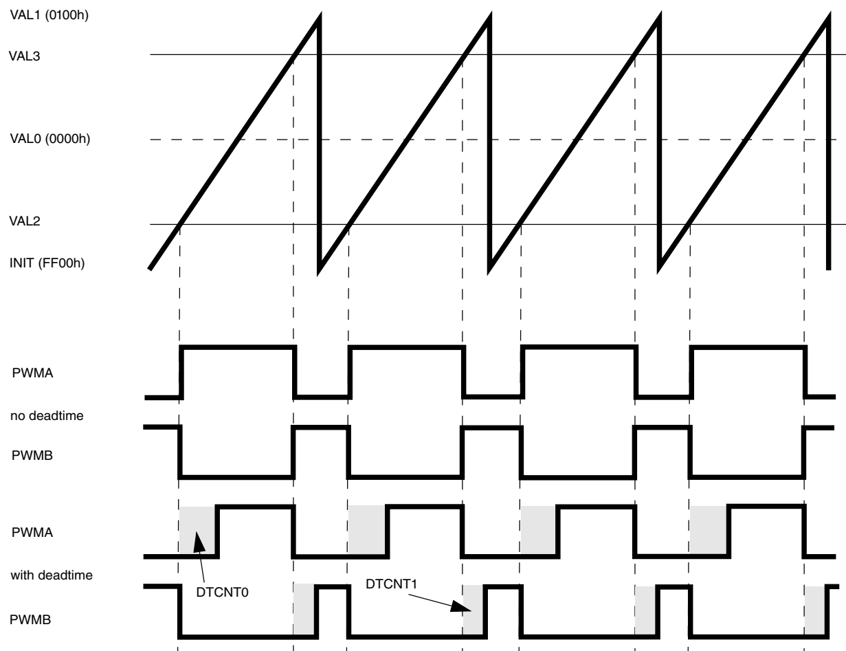
Figure 40-21. Deadtime Insertion
