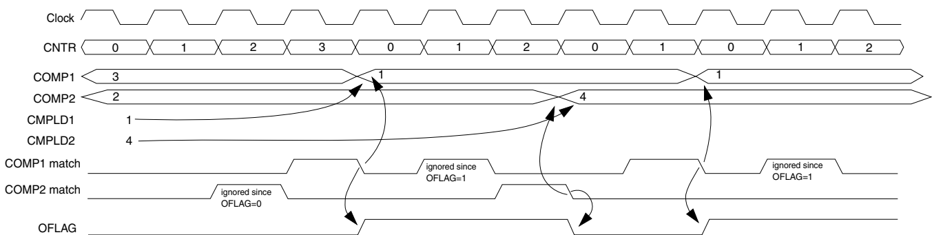
Figure 39-7. Variable PWM Waveform
