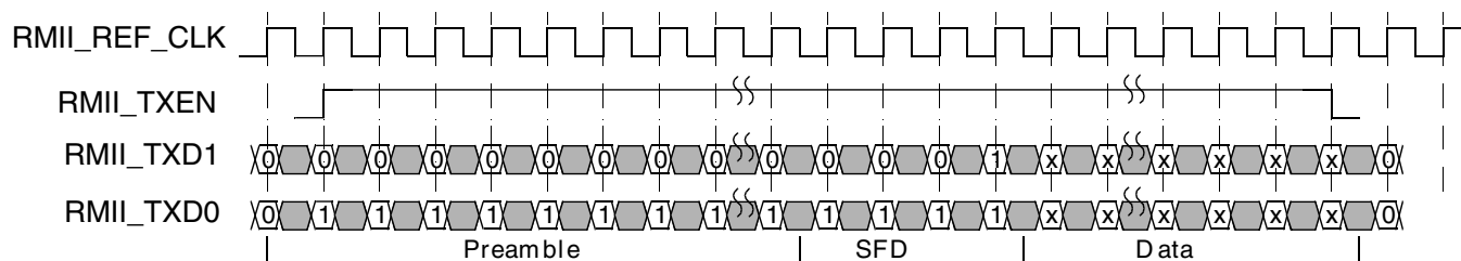
Figure 53-21. RMI transmit operation
