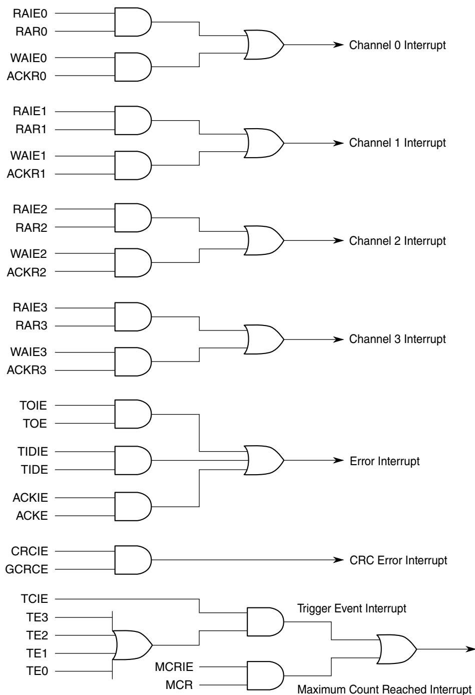
Figure 47-29. Interrupt description
