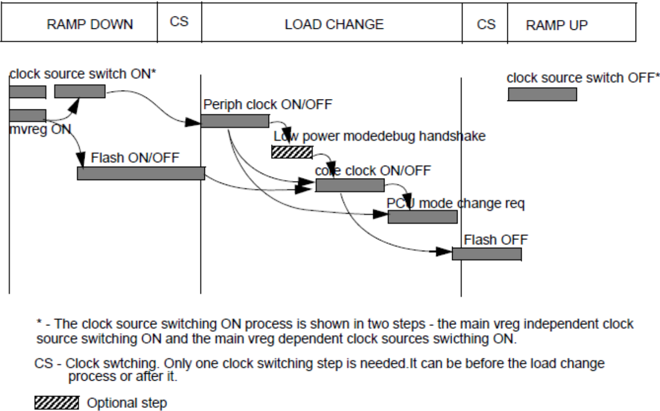
Figure 59-4. MC_ME mode transition process with PCS
