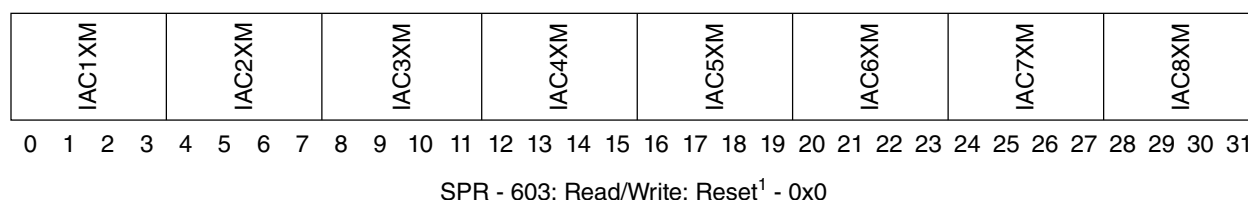
Figure 60-8. DBCR6 Register
