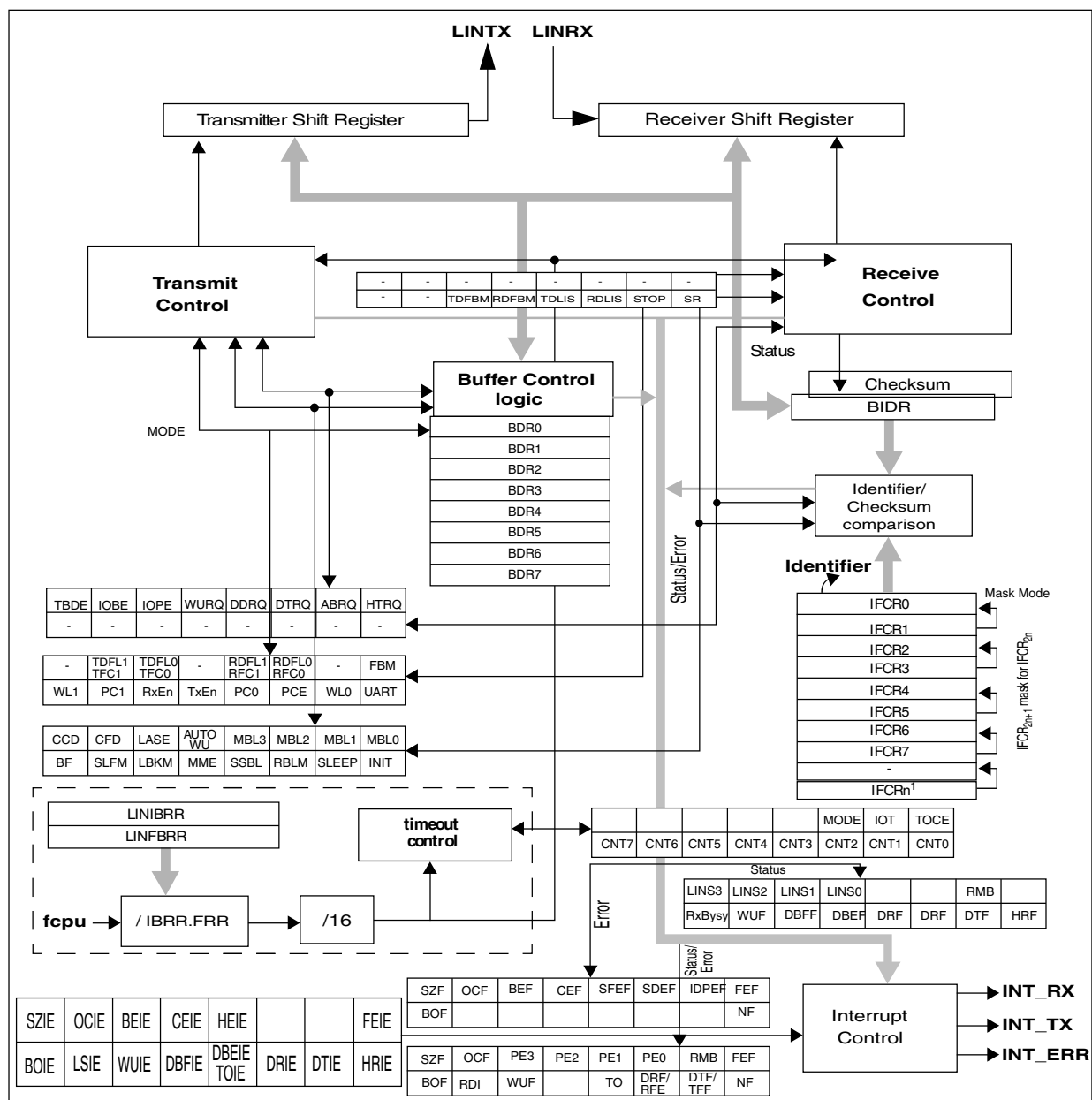
Figure 52-1. Block diagram
