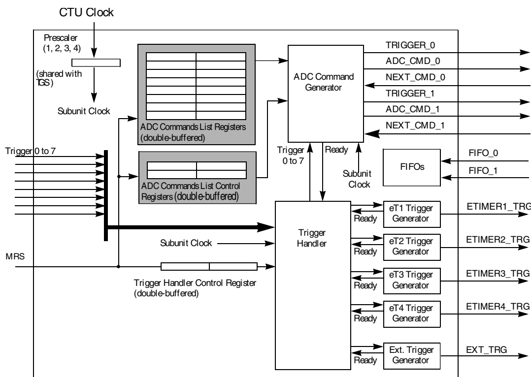
Figure 41-8. Scheduler subunit
