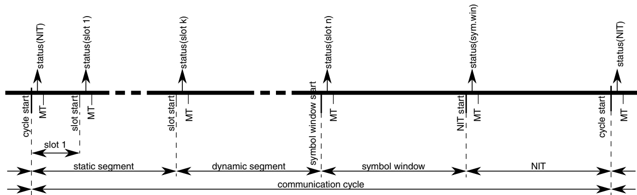
Figure 50-31. Slot Status Vector Update
