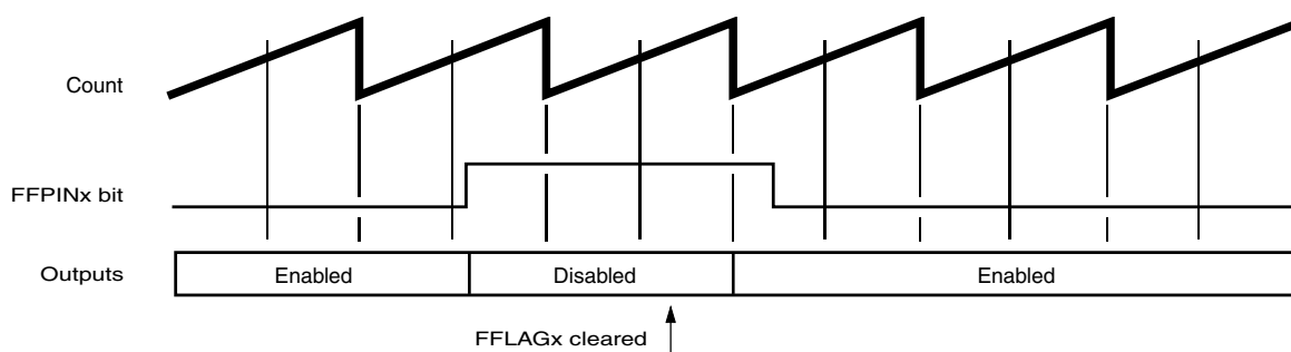
Figure 40-29. Manual Fault Clearing (FSAFE=0)
