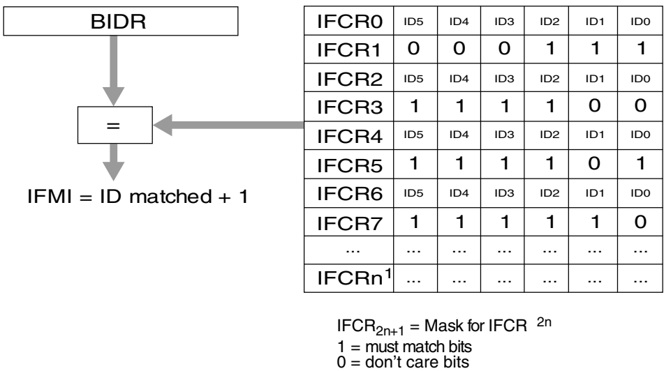
Figure 52-13. Identifier Mask mode
