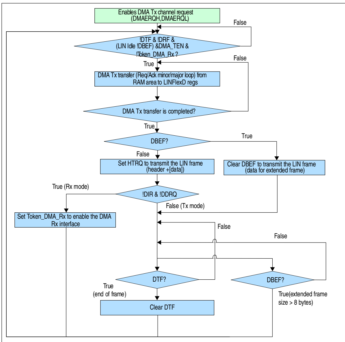
Figure 52-22. Master node – DMA Tx FSM (concept scheme)
