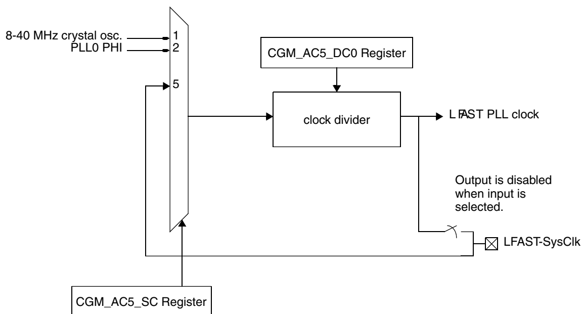
Figure 27-10. MC_CGM Auxiliary Clock 5 Generation Overview
