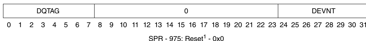
Figure 60-14. DEVENT Register
