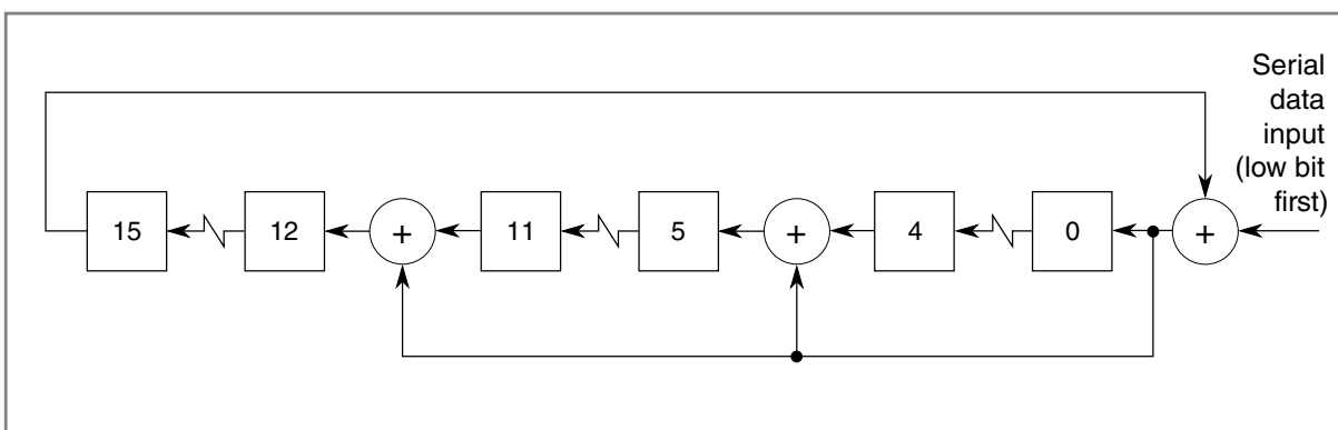
Figure 67-2. CRC-CCITT engine concept scheme
