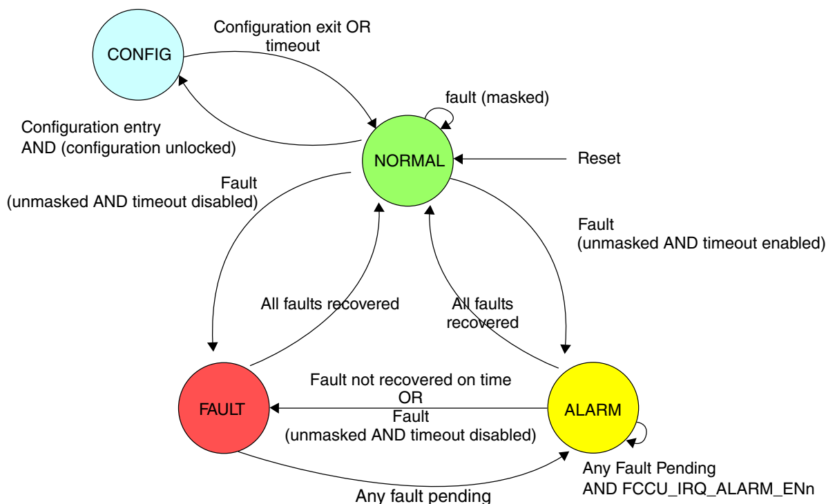
Figure 69-2. FCCU state diagram
