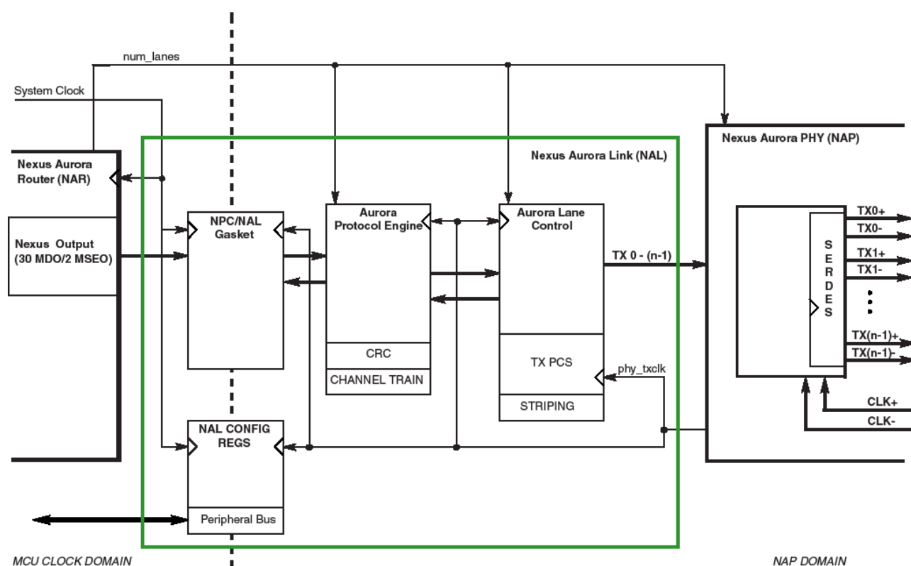
Figure 11-9. Aurora interface block diagram
