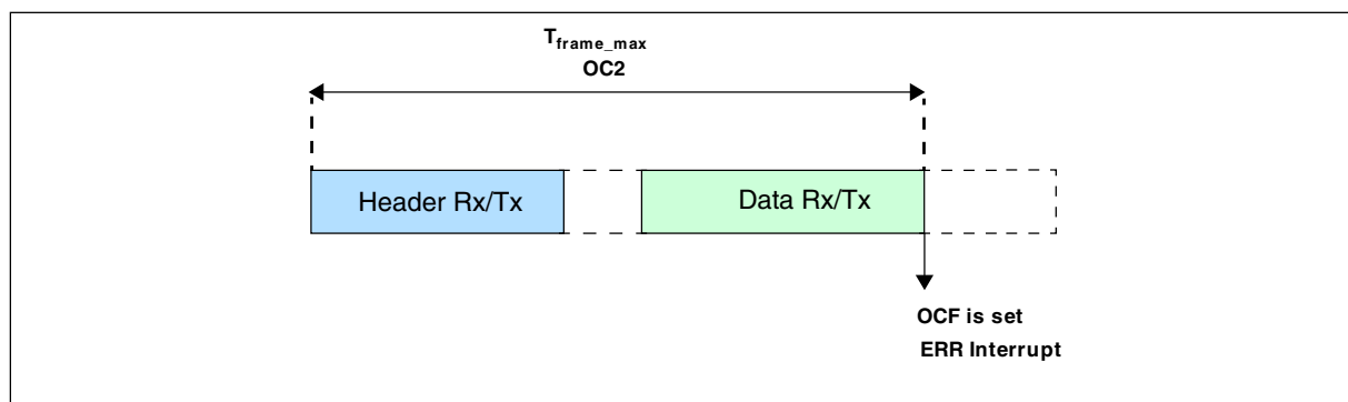
Figure 52-57. Frame timeout
