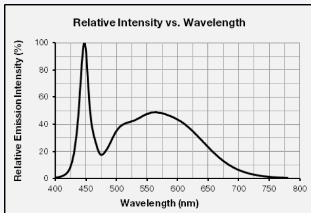
CCT: 5700 K
