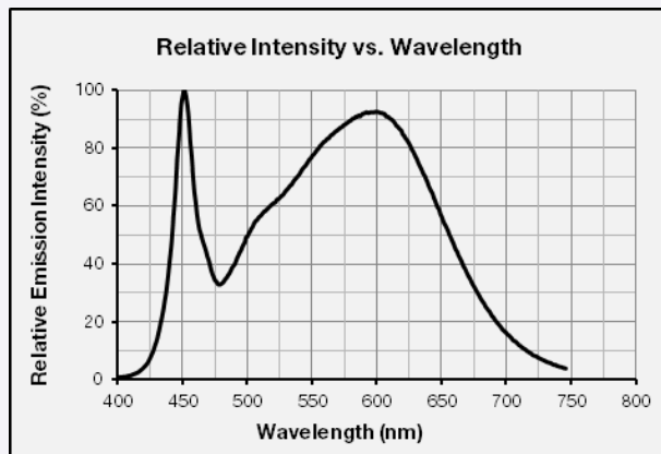
CCT: 4000 K
