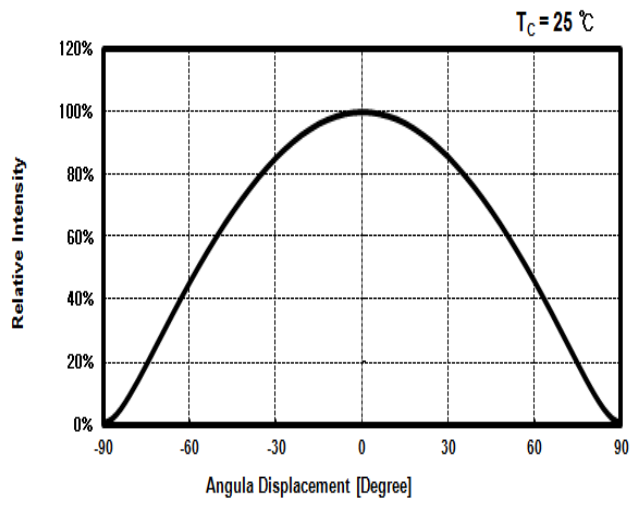
Radiation Pattern
