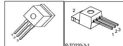
PG-TO262 PG-TO220
