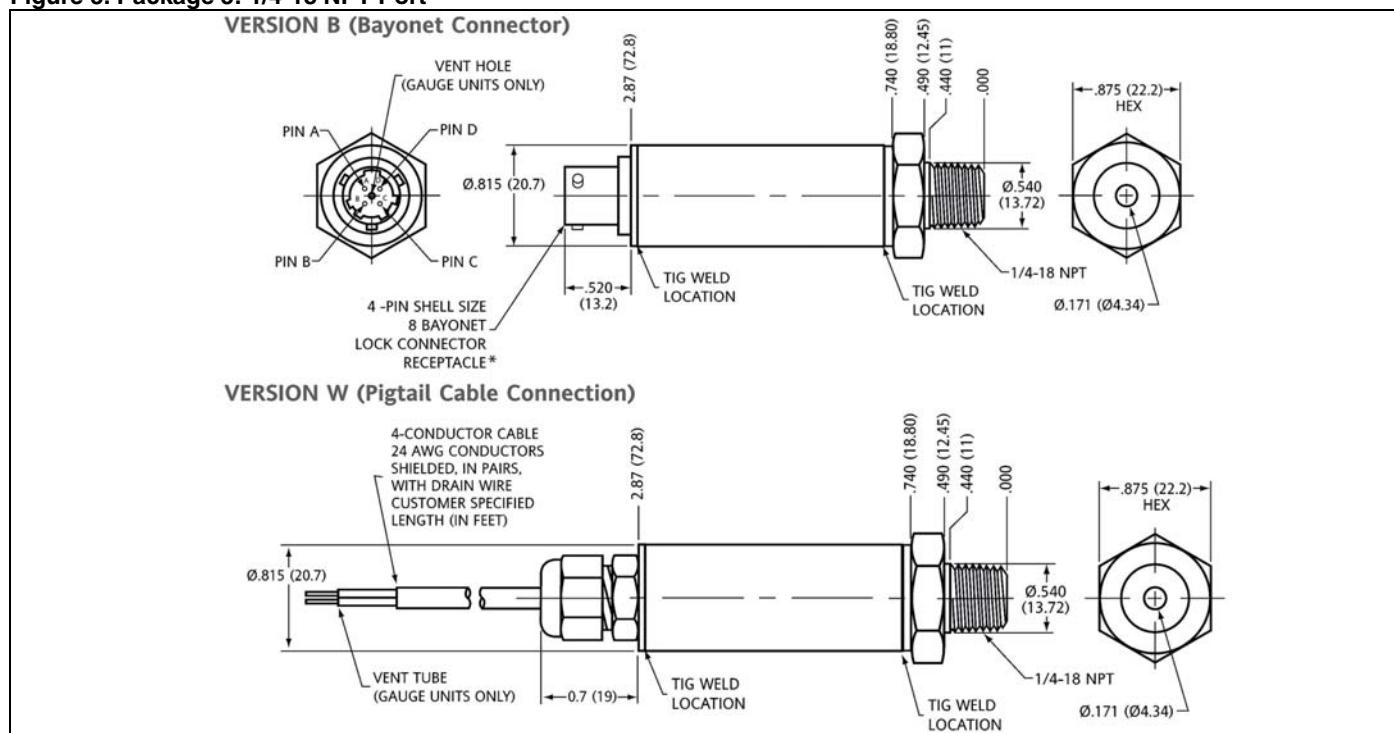
Figure 5. Package 5: 1/4-18 NPT Port
