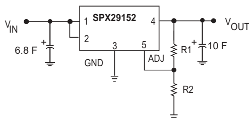
Figure 2. Adjustable Output Linear Regulator
