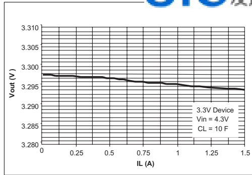
Figure 4. Load Regulation
