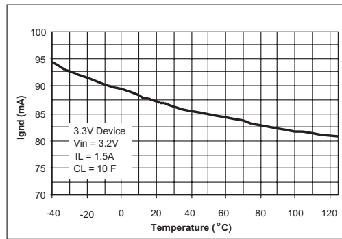
Figure 14. Output Current vs Temperature in Dropout at I_{LOAD}=1.5A
