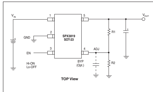
Figure 2. Typical Adjustable Output Voltage Configuration
