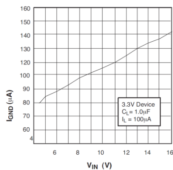
Fig. 4: Ground Current vs Input Voltage
