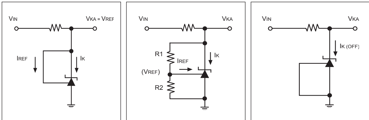
Test Circuit 1. Test Circuit for V_{KA} = V_{REF}
