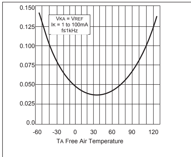
Low Frequency Dynamic Output Impedance vs. T AMBIENT
