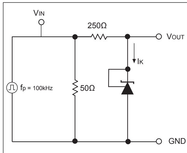
Test Circuit for Pulse Response
