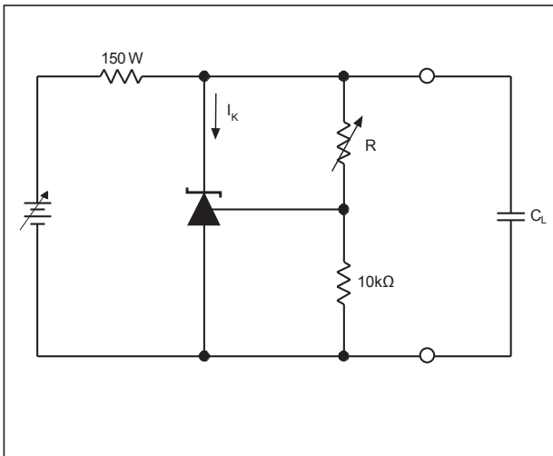
Test Circuit for Stability
