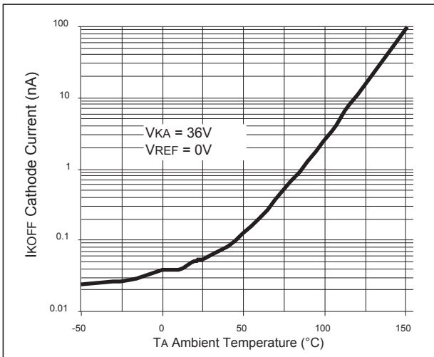
Off-State Leakage
