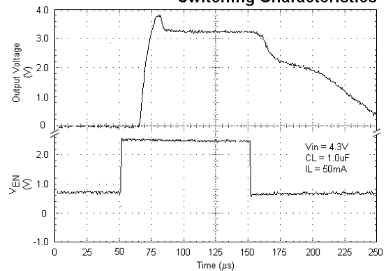
Switching Characteristics
