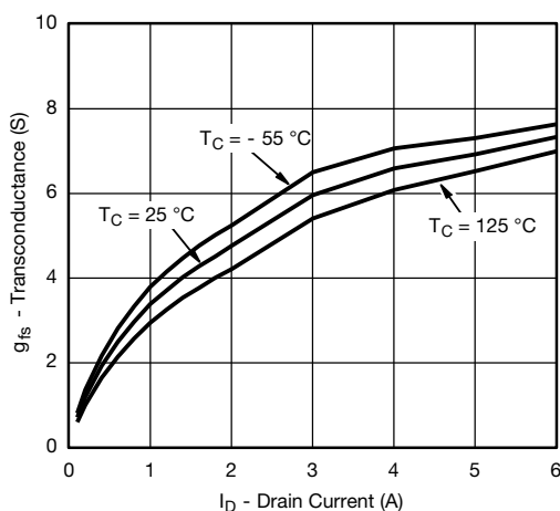
Transconductance
